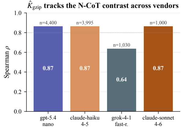
Figure 6: Spearman correlation between gzip \hat{K}_C and the N-CoT contrast indicator across the four-generator quartet. Three of four generators show \rho \approx 0.87 , with grok-4-1-fast-reasoning at \rho = 0.64 . All correlations are highly significant.
