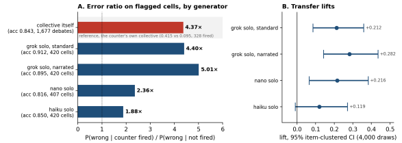
Figure 5: Transfer of the counter. (A) Ratio of the error rate on flagged to unflagged cells of item and framing, and debates for the collective, for the collective itself and for four solo generators the flag never touched. (B) Item-clustered intervals and point estimates on the four transfer lifts.
