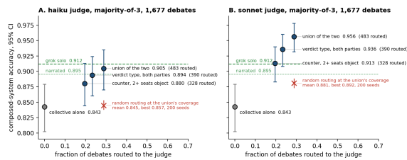
Figure 6: Composed-system accuracy against the fraction of debates routed to the judge, for the counter, the verdict-type router and the union, with random routing at the union’s coverage and the two solo grok baselines marked. Panel A routes to the haiku judge and panel B to the sonnet judge of the second design.
