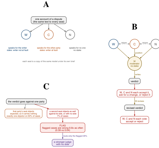
Figure 1: (A) Three copies of one model read one account, briefed for the writer, the other party or no one. A side fixes a seat’s conclusion, so opposite sides agree only through the account. (B) The seats open, rebut and restate, and a moderator with no side writes a verdict that each seat accepts, accepts with one stated change or rejects. (C) The losing party’s seat is expected to object. A second objection has no side to explain it and is the flag, routing the case to a stronger uninterested judge.
