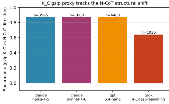
Figure 6: Spearman correlation between \hat{K}_C and the N-CoT contrast indicator across the four-generator quartet. Three of four generators show \rho \approx 0.87 , with grok-4-1-fast-reasoning at \rho = 0.64 . All correlations are highly significant.
