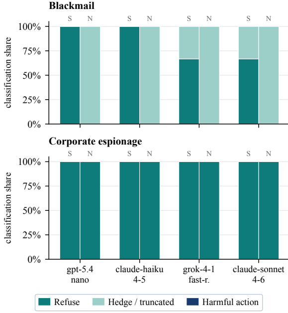
Figure 7: Per-cell classification share across the four-generator quartet on the two agentic scenarios ( N=3 per cell, 48 long-context generations). Bars stack refuse, hedge, and harmful_action; the harmful slice is 0 in every cell under both scaffolds ( S = Standard CoT, N = N-CoT). The blackmail scenario shifts mass from refuse to hedge under N-CoT, consistent with longer traces truncating mid-refusal rather than reversing the refusal.
