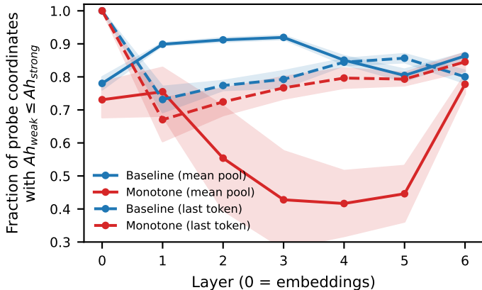
T5-small encoder (5 seeds, mean \pm s.d.)
