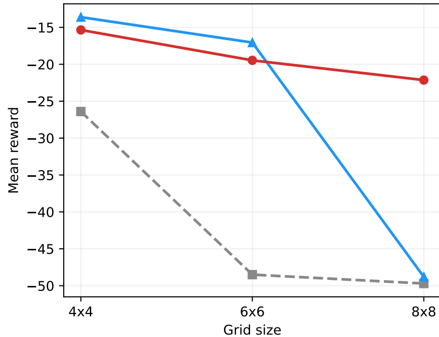
(b) Reward vs grid size
