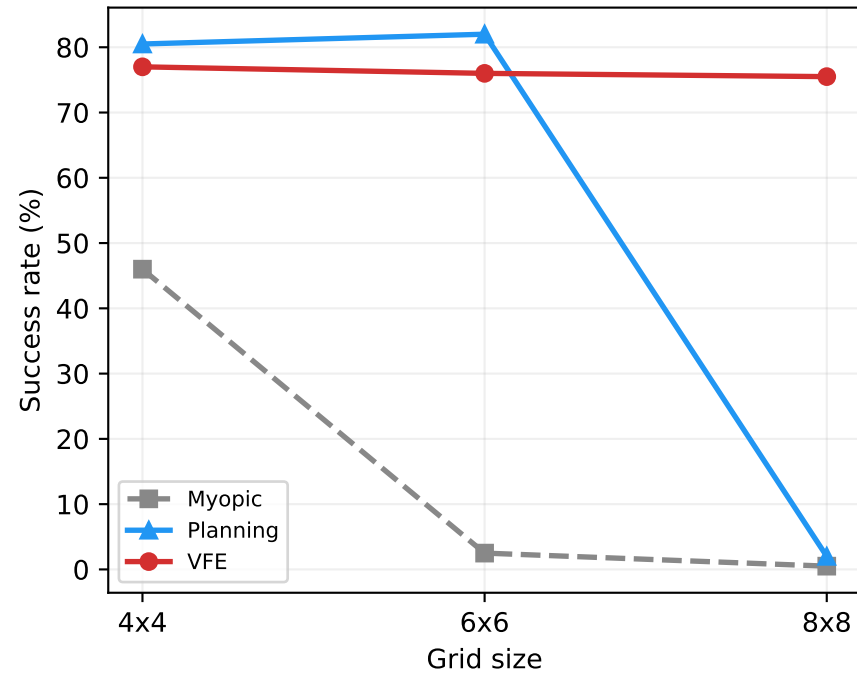
(a) Success rate vs grid size
