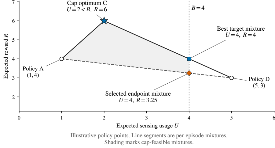
Fig. 3. An expected-usage target and a usage cap answer different questions. This schematic uses three illustrative policies and their per-episode mixtures, not benchmark data. The target U = B is the vertical line, while the shaded portion of the mixture hull satisfies the cap U \leq B . Suppose increasing grid weights select policies C, A, then D, so A and D form the selected crossing pair. A selected endpoint mixture can meet the target yet earn less than another mixture at the same usage. The highest-return cap-feasible policy can also leave part of the budget unused. These possibilities explain why calibration alone supplies neither an equality-constrained nor a cap-constrained reward optimum. They do not assert that every instance has either shortfall.
