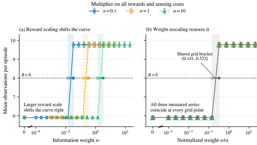
Fig. 4. Reward-scale transfer on Diagnosis. In (a), separately evaluated usage curves shift when rewards and sensing costs are multiplied by \alpha \in \{0.1, 1, 10\} . In (b), plotting against w/\alpha collapses them exactly, including the B=8 grid bracket (0.141, 0.323] . Points and error bars are means \pm 1 seed-level SE over five seeds and 100 episodes per seed, with shared per-episode streams. Lines guide the eye. Bands and open-closed endpoints mark grid brackets, not uncertainty intervals or policies attaining the target. The crossing between sampled points remains unresolved.
