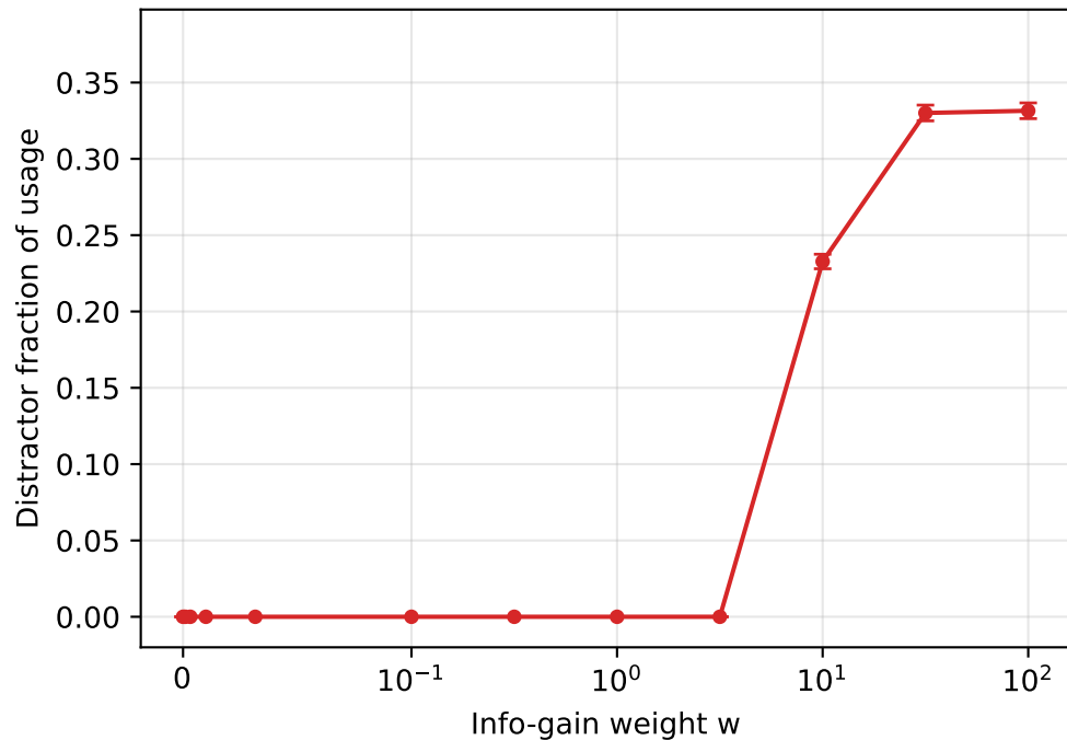
Reward-blind IG spends budget on the distractor
