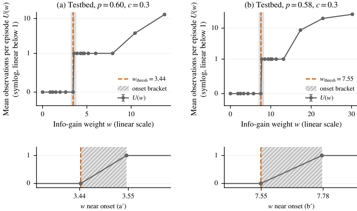
Fig. 23. Onset of observing on positive-threshold testbeds. The vermilion dashed vertical line marks the H=1 closed-form threshold (Proposition U.1) and the hatched gray band is the empirical onset bracket after grid refinement, magnified in the zoom row beneath each main panel, with the shaded strip on the main panel marking exactly the region the zoom row below it shows.
