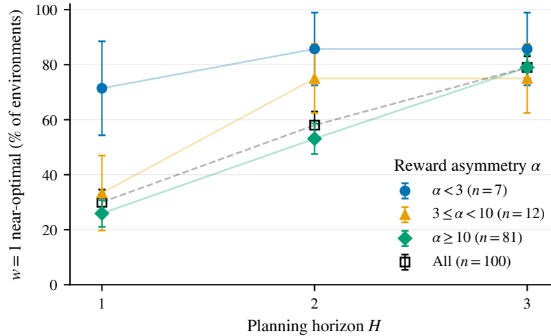
Fig. 17. Fraction of randomly generated two-state environments where w=1 is near-optimal, as a function of planning horizon H , stratified by reward asymmetry \alpha . The near-optimality basin widens with horizon, consistent with multi-step planning amplifying the value of observation. 100 environments, \alpha \in [1, 50] , p \in [0.55, 0.95] , cost \in [0.1, 5] . Markers show the three measured horizons H \in \{1, 2, 3\} with binomial standard-error bars, the legend reports the number of environments in each \alpha stratum, and the light guide lines connect measured points only.
