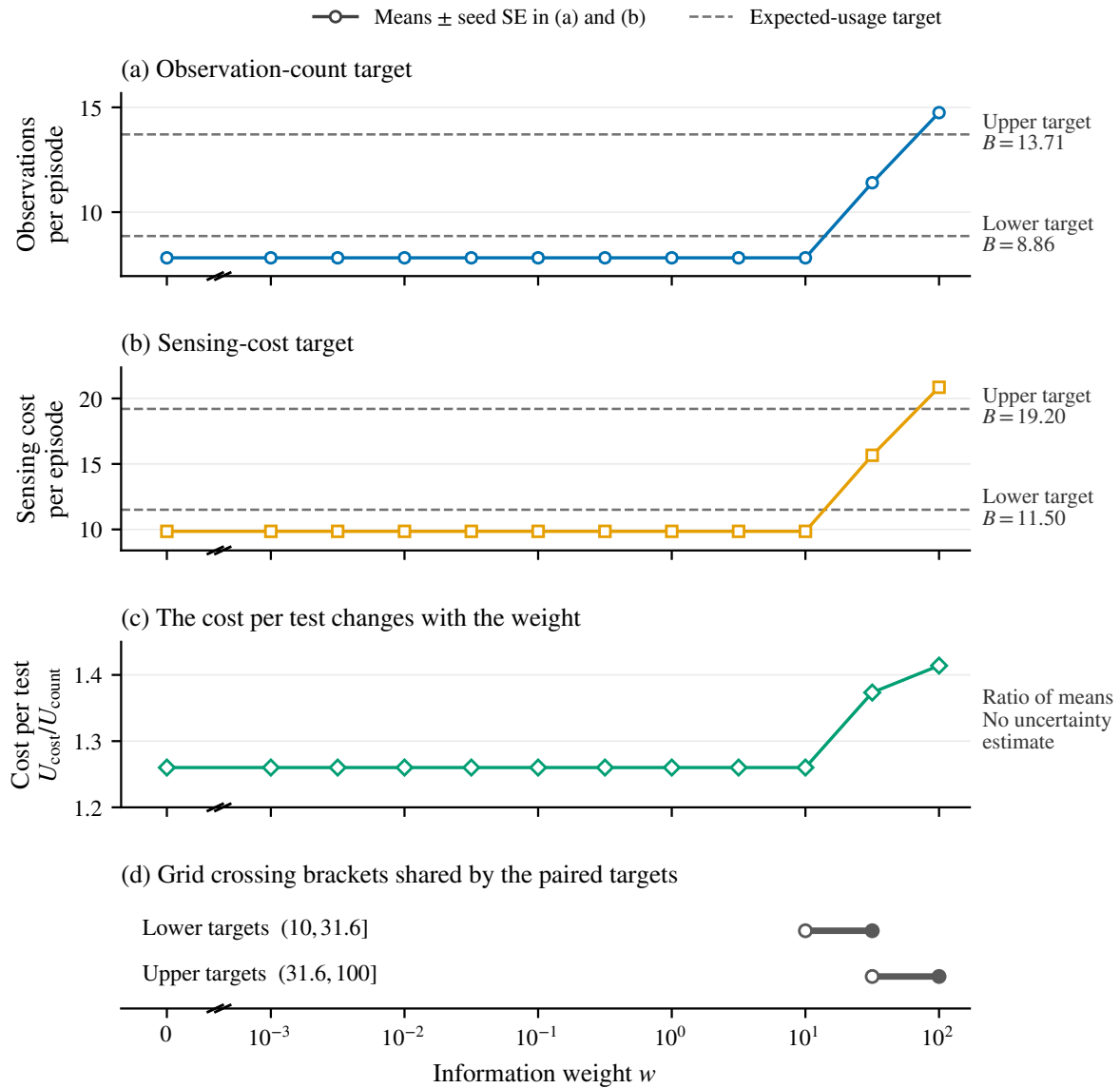
Fig. 22. Observation-count and sensing-cost targets on heterogeneous-cost Diagnosis. Panels (a) and (b) separate the two usage units, showing means \pm 1 seed-level SE and the tested targets as dashed lines. The lower count/cost targets are 8.86/11.50, and the upper targets are 13.71/19.20. Panel (c) shows the ratio of mean sensing cost to mean observation count, which rises as the test mix changes. No uncertainty estimate is shown for this ratio. Panel (d) displays the paired targets' shared crossing brackets, (10, 31.6] and (31.6, 100] . These intervals measure grid resolution, not statistical uncertainty. Lines joining sampled means guide the eye.
