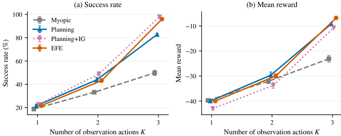
Fig. 12. Observation action scaling on Diagnosis ( N=8 , H=3 , 500 episodes). EFE separates from Planning only once several tests complete. The gap is zero at K=1 (bit-identical policies), -0.6\text{pp} and within seed-level sampling error at K=2 , and +13.2\text{pp} at K=3 , where choosing among differentially informative tests is exactly what the information-gain term contributes. InfoGain-Tuned is not part of this battery, so the legend carries four agents rather than the five of Figure 14.
