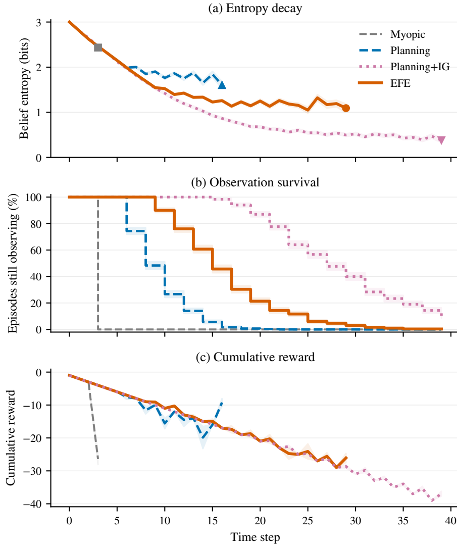
Fig. 16. Exploration efficiency on Diagnosis ( N=8 , K=3 , 300 episodes). (a) Belief entropy decay. (b) Percentage of episodes still observing. (c) Cumulative reward. Panels are stacked on a shared time axis, shaded bands show \pm 1 SE across episodes, and in panel (a) a marker terminates each series at its final plotted step. Panels (a) and (c) average, at each step, only the episodes still running at that step. Planning+IG uses the myopic Info Gain agent's success-tuned weight, selected on 100 tuning episodes and transferred to Planning+IG for this visualization, not the own-class tuning protocol of the main tables (Section 3). EFE stops observing later than reward-only Planning and earlier than Planning+IG, whose survival curve lies at or above EFE's at every step (panel b).
