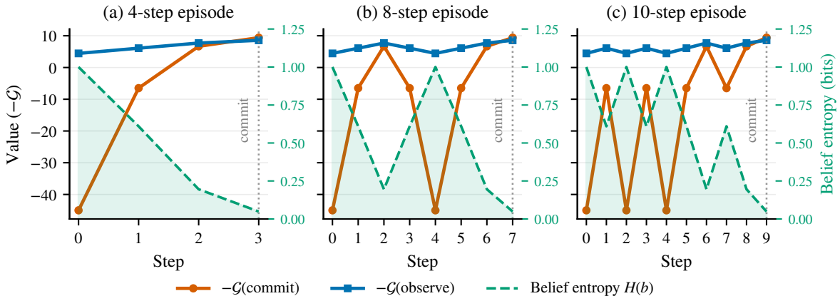
Fig. 11. EFE decomposition within Tiger episodes ( H=6 ). The agent commits at the crossover where commit value (circles) exceeds observe value (squares). As belief entropy (dashed line with shading) decreases, the transition from exploration to exploitation occurs automatically.
