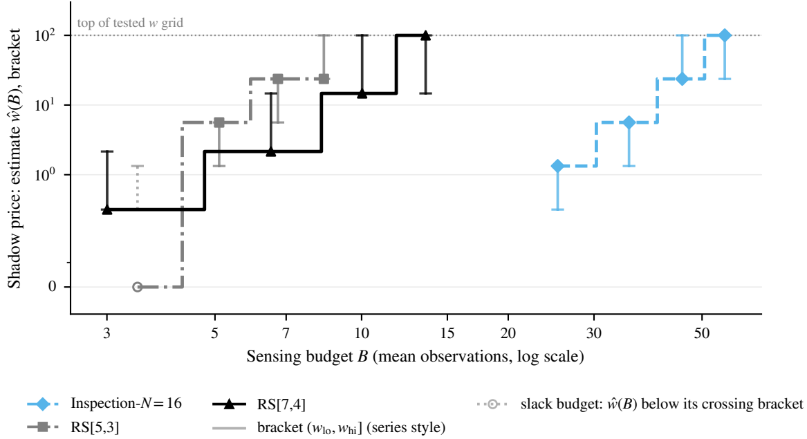
Fig. 24. Grid estimates of the shadow price on three interleaved (non-observe-then-commit) settings, RockSample[5,3], RockSample[7,4], and Inspection- N=16 , with crossing brackets marked as vertical bars, capped where they reach the dotted rule marking the top of the tested w grid, and an open-circle marker where a budget is slack (the grid weight whose usage comes nearest to the budget sits strictly below the bracket's lower edge, here w=0 on the lowest RockSample[5,3] budget). Every marker plots the nearest-point solution \hat{w}(B) , which can sit on a bracket's lower edge. The budget axis is logarithmic and the weight axis uses a symmetric-log scale, linear near zero. The underlying usage curves U(w) are monotone at every sampled grid point on RockSample[7,4] and Inspection- N=16 , while RockSample[5,3] dips once near w=0.316 before rising (see text).
