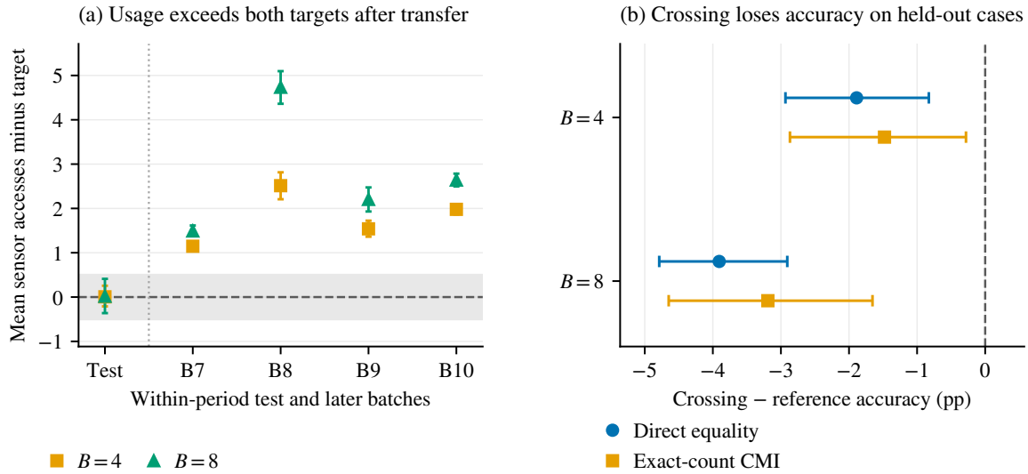
Fig. 6. Usage transfer and accuracy costs on recorded sensor cases for the two available crossings, B = 4 and B = 8 . (a) Each point is mean usage minus its target on within-period test cases or one later batch. The gray band is the predeclared \pm 0.5 access tolerance. Test intervals have 98.333% conditional bootstrap coverage with calibration reselection; later intervals are nominal 95% with selections fixed. Collection groups are categorical, so points are not connected. (b) Paired test accuracy gaps against direct equality mixtures and exact-count greedy conditional-information acquisition (CMI), with nominal 95% intervals including calibration reselection. Positive gaps favor the crossing mixture. Direct mixtures need not exactly meet B on test cases. All intervals condition on one fitted model and within-stratum case exchangeability. The fixed B = 2 request has no calibration crossing and fails the all-target criterion; it is stated here rather than plotted as a measurement.
