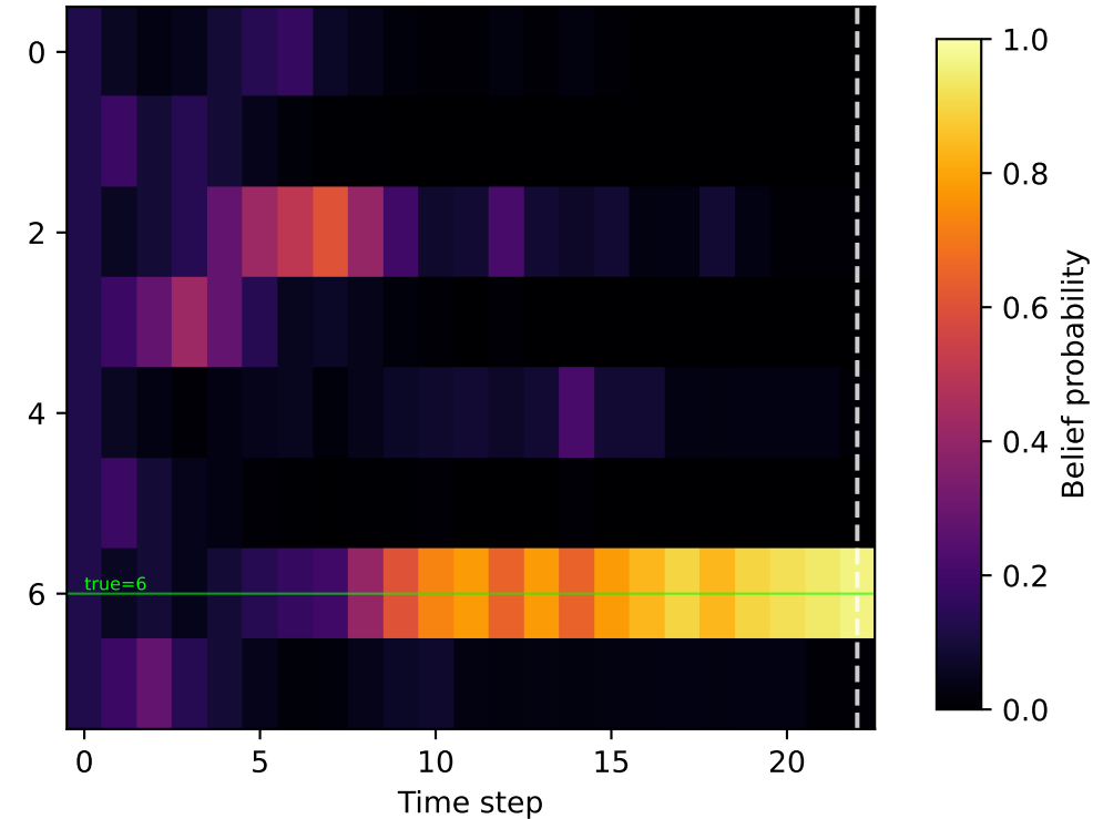
(c) InfoGain-Tuned obs=22, correct, R=-12.0
