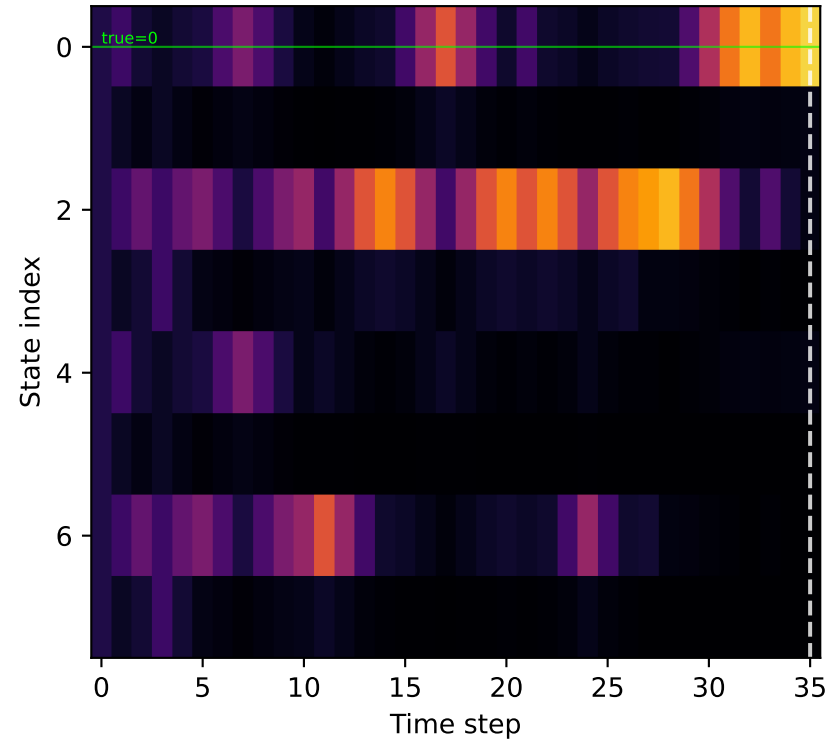
(a) VFE ( w = 1 ) obs=35, correct, R=-25.0
