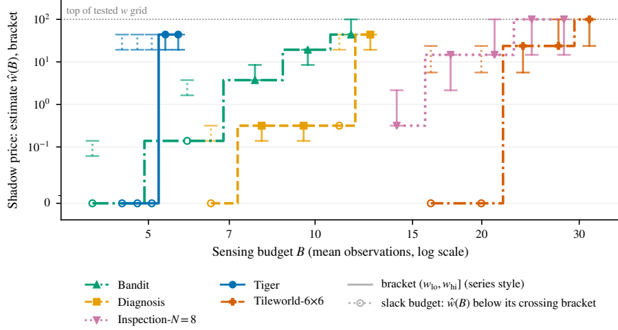
Fig. 5. Operational shadow-price staircases w^*(B) across five observe-then-commit and inspection domains (Tiger, Bandit, Diagnosis, Inspection- N=8 , Tileworld- 6 \times 6 ), each in its own color, with a logarithmic budget axis and a symmetric-log weight axis that is linear near zero. Each staircase steps up as the sensing budget B rises, and the vertical bar at each step marks that budget’s crossing bracket (w_{lo}, w_{hi}] (Definition 2), capped where the bracket’s upper edge coincides with the top of the tested w grid (dotted horizontal rule at 100). An open circle with a dotted bar marks a slack budget, one for which the grid weight whose usage comes nearest to the budget lies strictly below the lower edge of the crossing bracket ( w=0 at seven of the nine marked budgets, w=0.316 at Diagnosis B=11.06 , and w=0.139 at Bandit B=5.87 , the twice-crossed budget discussed in the text), so the nearest-point solution returns a weight below the bracket while the dotted bar still marks the crossing. Every marker plots that nearest-point solution \hat{w}(B) , which can also sit on a bracket’s lower edge. The usage curves behind Tiger, Diagnosis, and Inspection never step downward between consecutive sampled weights, while Bandit and Tileworld show local non-monotonicity from discrete policy switches, so their brackets mark the last crossing of each budget by the convention of Definition 2.
