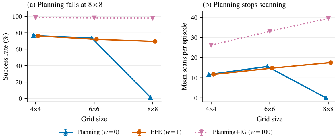
Fig. 9. Why fixed-depth Planning fails on the largest Tileworld grid ( H = 2 , 200 episodes per seed over five seeds). (a) Planning and EFE have similar success at 4x4 and 6x6, but at 8x8 Planning falls to 1.4% while EFE reaches 69.4%. (b) Planning takes no scans at 8x8, compared with EFE's 17.50 per episode. The fixed w = 100 Planning+IG comparator reaches 97.8% success using 39.52 scans, but earns -30.84 mean reward against EFE's -25.86 (reward not plotted). Panel (a) error bars are seed-level SE. Panel (b) shows mean scan counts without uncertainty bars. The other two agents, rewards, and timing measurements remain in results_tileworld_scaling.csv.
