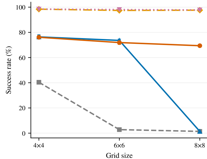
(a) Success rate vs grid size
