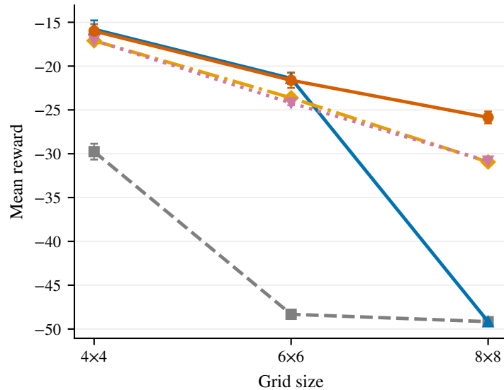
(b) Reward vs grid size
