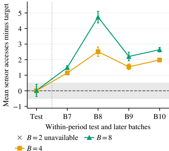
(a) Usage transfer 98.333% test / 95% later intervals
