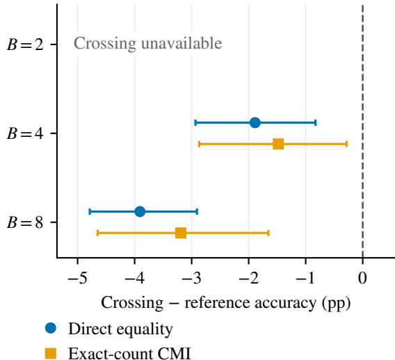
(b) Held-out accuracy gaps 95% paired intervals
