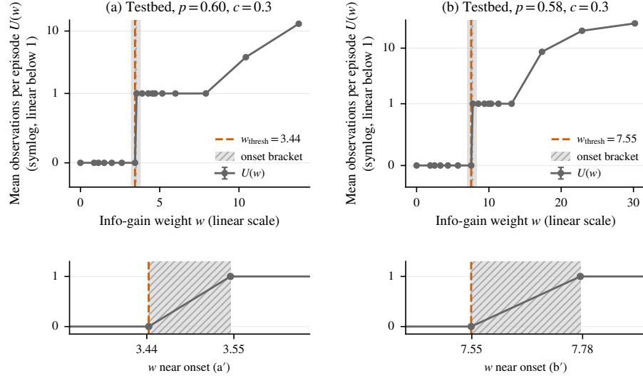
Fig. 23. Onset of observing on positive-threshold testbeds. The vermillion dashed vertical line marks the H=1 closed-form threshold (Proposition 6) and the hatched gray band is the empirical onset bracket after grid refinement, magnified in the zoom row beneath each main panel, with the shaded strip on the main panel marking exactly the region the zoom row below it shows.
