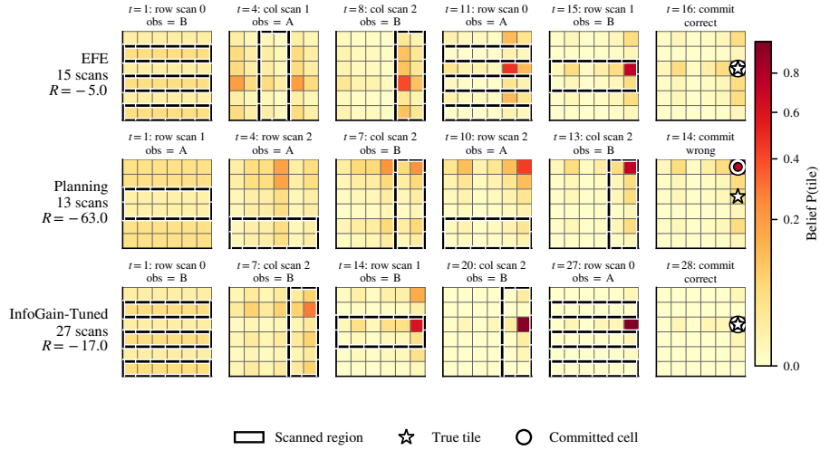
Fig. 25. Agent comparison on the same 6 \times 6 Tileworld episode. All agents start from the identical uniform prior, stated here rather than drawn once per row. Belief probability is encoded by the shared colorbar on a square-root color scale. Black outlines mark the cell group queried by each scan, each panel’s title reports that scan’s noisy binary readout as \text{obs}=\text{A} or \text{obs}=\text{B} naming which half of the queried group the signal favors, the black-edged white star marks the true tile, and the black-stroked white ring marks the committed cell. Scan panels are subsampled evenly within each row, so columns are not time-aligned across rows and each panel’s t gives the true step. EFE (top) commits correctly with efficient scanning. Planning (middle) commits on the wrong cell after 13 scans. InfoGain-Tuned (bottom) over-scans well past the point of diminishing returns.
