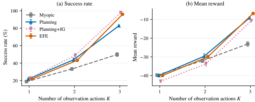
Fig. 12. Observation action scaling on Diagnosis ( N=8 , H=3 , 500 episodes). EFE separates from Planning only once several tests compete. The gap is zero at K=1 (bit-identical policies), -0.6\text{pp} and within seed-level sampling error at K=2 , and +13.2\text{pp} at K=3 , where choosing among differentially informative tests is exactly what the information-gain term contributes. InfoGain-Tuned is not part of this battery, so the legend carries four agents rather than the five of Figure 14.
