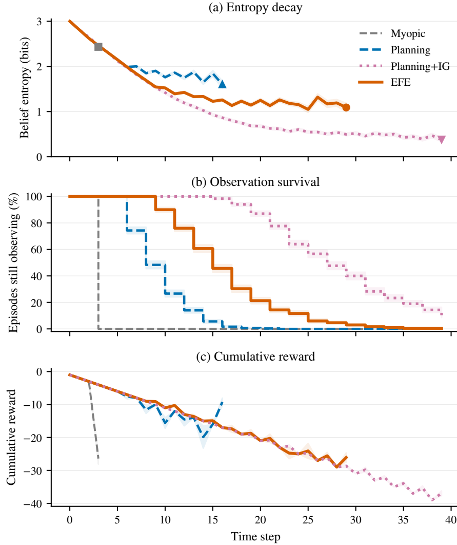
Fig. 16. Exploration efficiency on Diagnosis ( N=8 , K=3 , 300 episodes). (a) Belief entropy decay. (b) Percentage of episodes still observing. (c) Cumulative reward. Panels are stacked on a shared time axis, shaded bands show \pm 1 SE across episodes, and in panel (a) a marker terminates each series at its final plotted step. Panels (a) and (c) average, at each step, only the episodes still running at that step. Planning+IG uses the myopic Info Gain agent’s success-tuned weight, selected on 100 tuning episodes and transferred to Planning+IG for this visualization, not the own-class tuning protocol of the main tables (Section 3). EFE stops observing later than reward-only Planning and earlier than Planning+IG, whose survival curve lies at or above EFE’s at every step (panel b).
