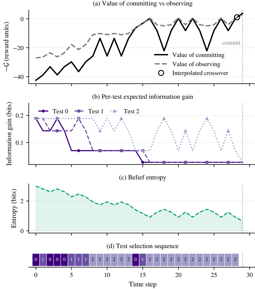
Fig. 13. EFE decomposition over an extended Diagnosis episode ( N=8 , K=3 ). (a) Value of committing vs. observing. The open circle marks the value crossover interpolated between sampled steps. The dotted vertical line marks the actual discrete commit step in all four panels. (b) Per-test expected information gain. Tests become differentially informative as belief concentrates, and the agent shifts its test selection as they do, though the recursive score it optimizes is not the one-step information gain plotted here. (c) Belief entropy decay. (d) Test selection sequence showing the agent's adaptive strategy.
