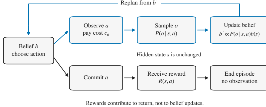
Fig. 19. The observe-then-commit decision loop, shown schematically. An observation incurs a cost and updates the belief about a hidden state that remains fixed. The agent then chooses again from the updated belief. A commit instead pays a state-dependent reward and ends the episode without emitting an observation. Rewards are not inputs to the belief update. The loop describes the episode, while the planner’s finite horizon limits how far it looks ahead at each decision.
