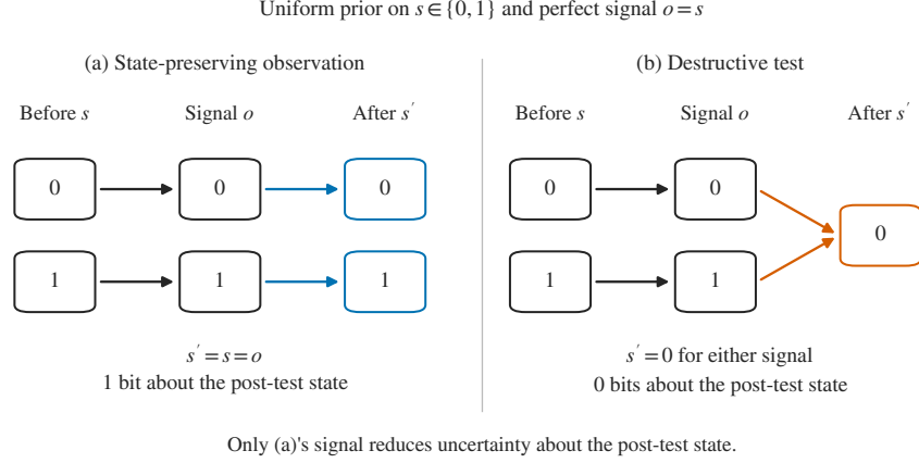
Fig. 20. An observation can describe a state that no longer exists. These schematic timelines use a perfect sensor to contrast state-preserving sensing with the destructive test of Example 1. The sensor reports the pre-action state in both cases. Under preservation that report identifies the state used by the next decision. Under destruction both possible initial states become 0, so the correct post-action belief is (1, 0) for either report. Treating a report of 1 as the current state gives an obsolete posterior. The example limits the state-preserving reduction, not transition-aware EFE.
