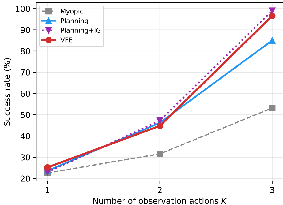
(a) Success vs. observation action complexity
