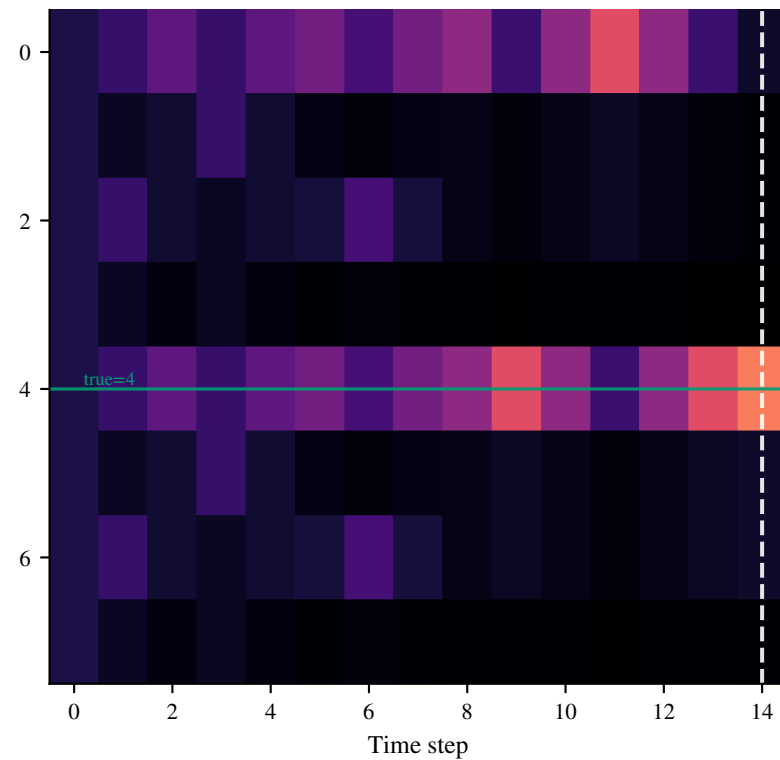
(b) Planning ( \rho = 0 ) obs=14, correct, R=-4.0
