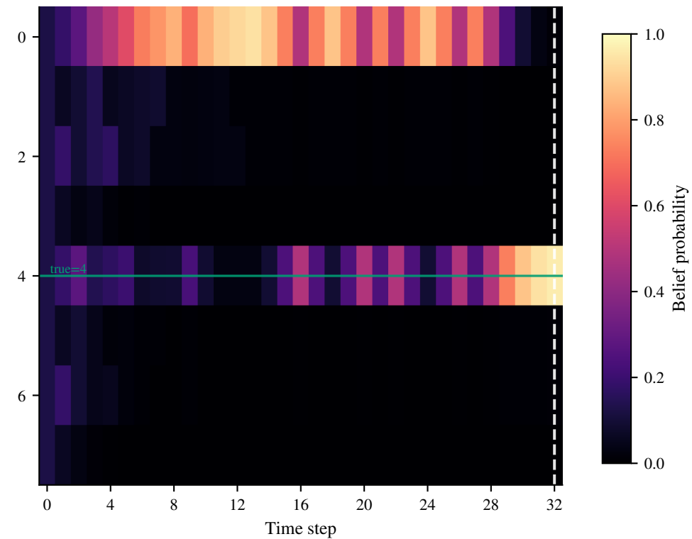
(c) InfoGain-Tuned obs=32, correct, R=-22.0
