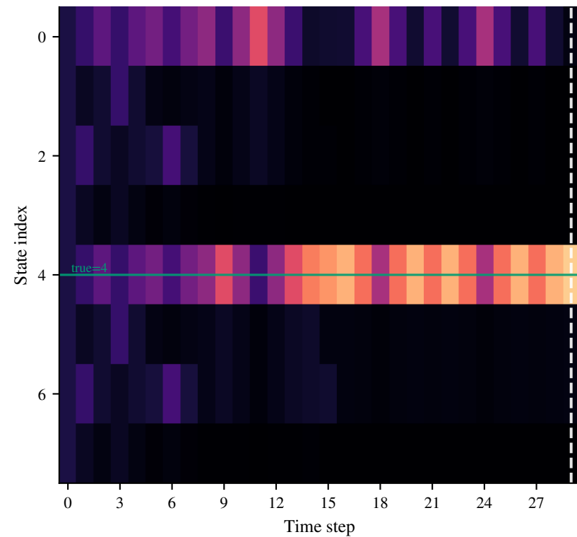
(a) EFE ( w = 1 ) obs=29, correct, R=-19.0
