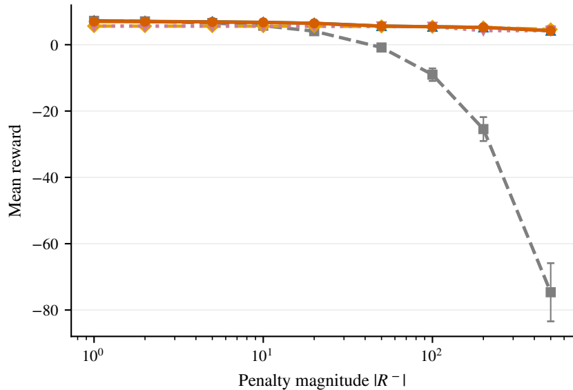
(b) Reward vs. reward asymmetry
