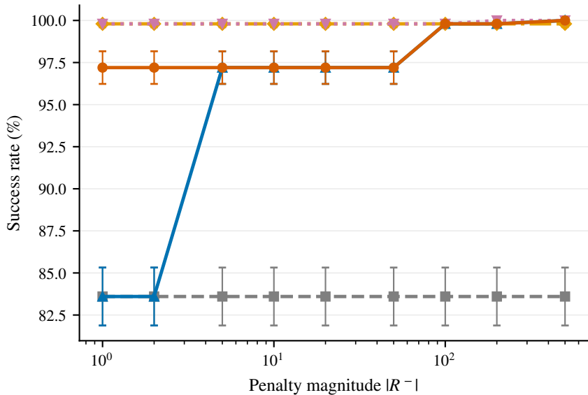
(a) Success rate vs. reward asymmetry
