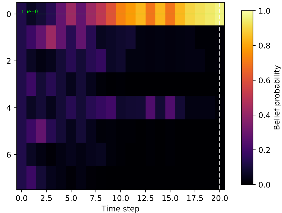
(c) InfoGain-Tuned obs=20, correct, R=-10.0
