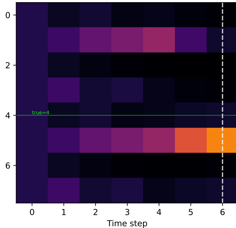
(b) Planning ( \rho = 0 ) obs=6, wrong, R=-56.0
