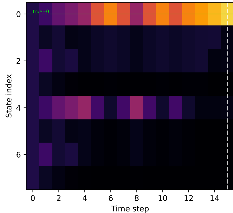
(a) EFE ( w = 1 ) obs=15, correct, R=-5.0
