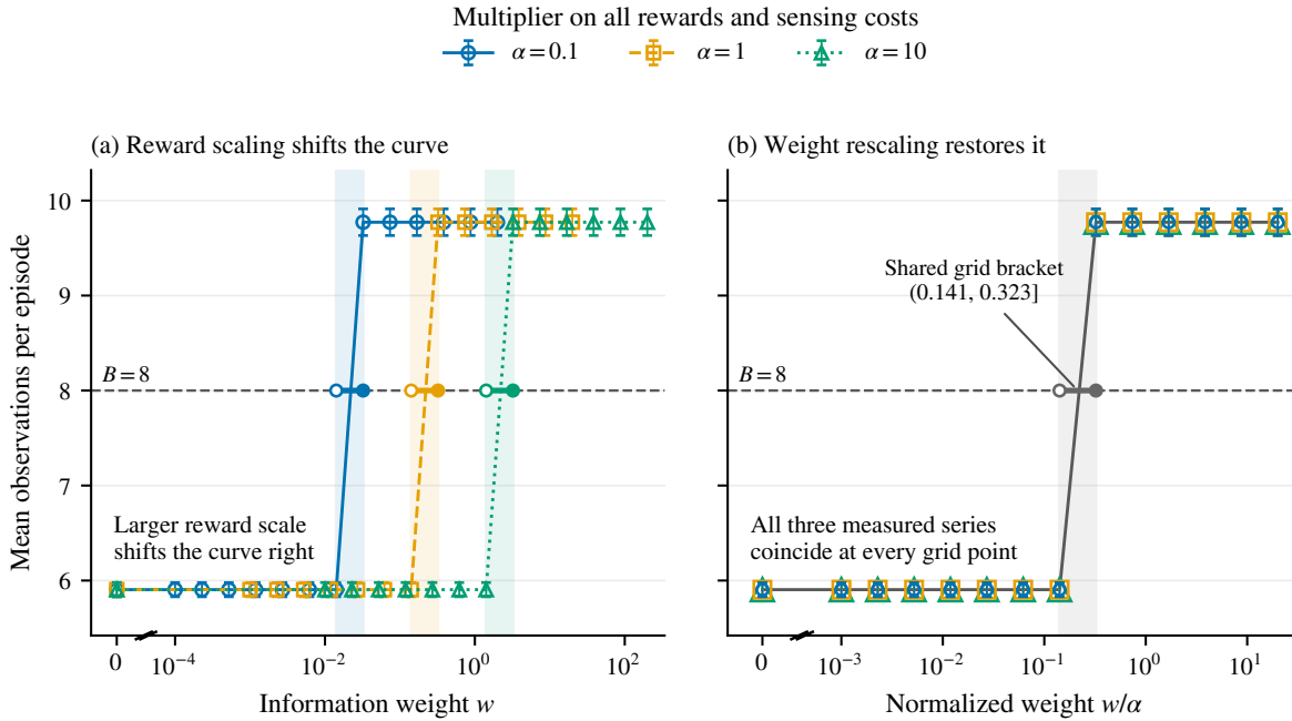
Fig. 5. Reward-scale transfer on Diagnosis. In (a), separately evaluated usage curves shift when rewards and sensing costs are multiplied by \alpha \in \{0.1, 1, 10\} . In (b), plotting against w/\alpha collapses them exactly, including the B=8 grid bracket (0.141, 0.323] . Points and error bars are means \pm 1 seed-level SE over five seeds and 100 episodes per seed, with shared per-episode streams. Lines guide the eye. Bands and open-closed endpoints mark grid brackets, not uncertainty intervals or policies attaining the target. The crossing between sampled points remains unresolved.
