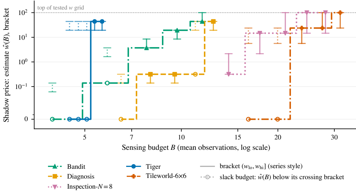
Fig. 9. Operational shadow-price staircases w^*(B) across five observe-then-commit and inspection domains (Tiger, Bandit, Diagnosis, Inspection- N=8 , Tileworld-6x6), each in its own color, with a logarithmic budget axis and a symmetric-log weight axis that is linear near zero. Each staircase steps up as the sensing budget B rises, and the vertical bar at each step marks that budget's crossing bracket (w_{lo}, w_{hi}) (Definition 4.1), capped where the bracket's upper edge coincides with the top of the tested w grid (dotted horizontal rule at 100). An open circle with a dotted bar marks a slack budget, one for which the grid weight whose usage comes nearest to the budget lies strictly below the lower edge of the crossing bracket ( w=0 at seven of the nine marked budgets, w=0.316 at Diagnosis B=11.06 , and w=0.139 at Bandit B=5.87 , the twice-crossed budget discussed in the text), so the nearest-point solution returns a weight below the bracket while the dotted bar still marks the crossing. Every marker plots that nearest-point solution \hat{w}(B) , which can also sit on a bracket's lower edge. The usage curves behind Tiger, Diagnosis, and Inspection never step downward between consecutive sampled weights, while Bandit and Tileworld show local non-monotonicity from discrete policy switches, so their brackets mark the last crossing of each budget by the convention of Definition 4.1.
