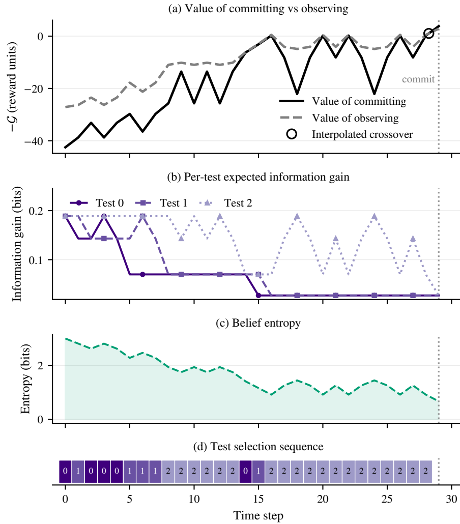
Fig. 15. EFE decomposition over an extended Diagnosis episode ( N=8, K=3 ). (a) Value of committing vs. observing. The open circle marks the value crossover interpolated between sampled steps. The dotted vertical line marks the actual discrete commit step in all four panels. (b) Per-test expected information gain. Tests become differentially informative as belief concentrates, and the agent shifts its test selection as they do, though the recursive score it optimizes is not the one-step information gain plotted here. (c) Belief entropy decay. (d) Test selection sequence showing the agent's adaptive strategy.
