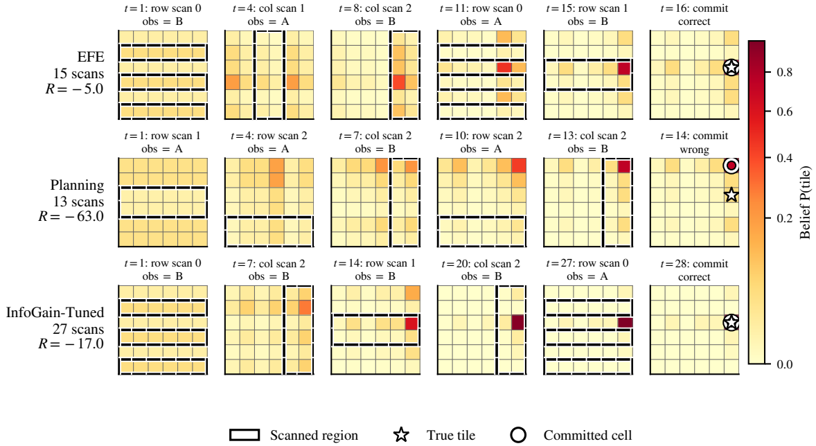
Fig. 25. Agent comparison on the same 6x6 Tileworld episode. All agents start from the identical uniform prior, stated here rather than drawn once per row. Belief probability is encoded by the shared colorbar on a square-root color scale. Black outlines mark the cell group queried by each scan, each panel's title reports that scan's noisy binary readout as obs=A or obs=B naming which half of the queried group the signal favors, the black-edged white star marks the true tile, and the black-stroked white ring marks the committed cell. Scan panels are subsampled evenly within each row, so columns are not time-aligned across rows and each panel's t gives the true step. EFE (top) commits correctly with efficient scanning. Planning (middle) commits on the wrong cell after 13 scans. InfoGain-Tuned (bottom) over-scans well past the point of diminishing returns.
