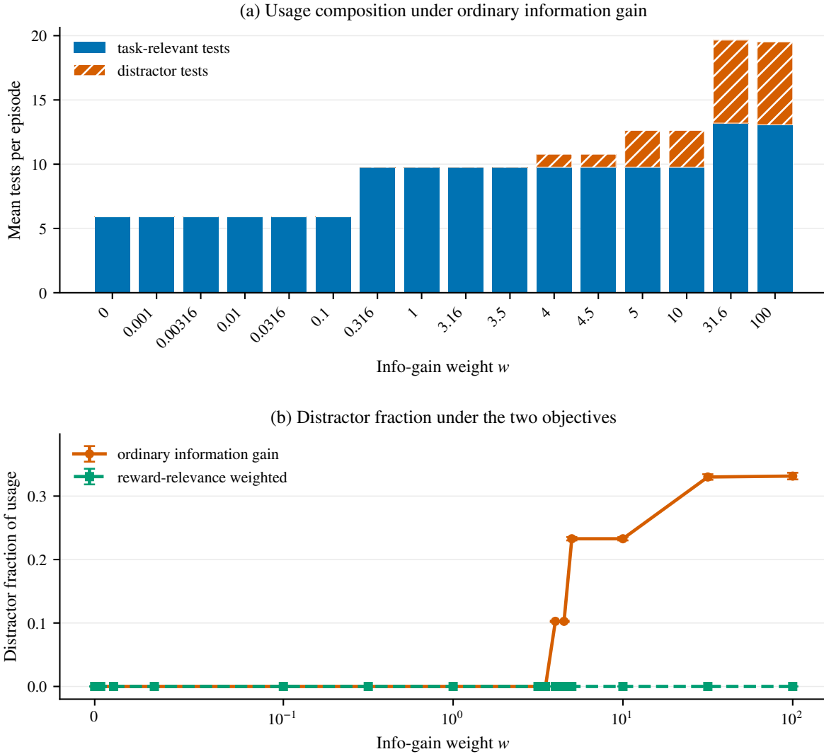
Fig. 10. Reward-irrelevant sensing on DistractorDiagnosisEnv. The upper panel decomposes ordinary Planning+IG’s usage into task-relevant and distractor tests as w grows. Distractor spend is zero below the onset bracket (3.5, 4.0] and saturates at roughly a third of total usage. The lower panel plots the distractor fraction for ordinary information gain against the reward-relevance-weighted variant on the same grid. The weighted variant is flat at exactly zero everywhere. Error bars are seed-level SE over 5 seeds.
