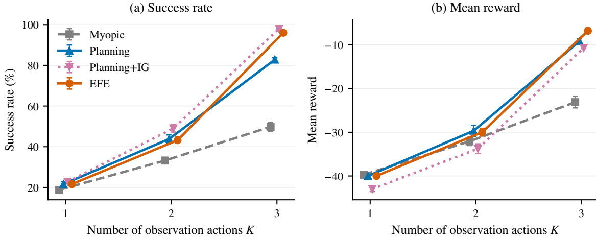
Fig. 14. Observation action scaling on Diagnosis ( N=8 , H=3 , 500 episodes). EFE separates from Planning only once several tests compete. The gap is zero at K=1 (bit-identical policies), -0.6 pp and within seed-level sampling error at K=2 , and +13.2 pp at K=3 , where choosing among differentially informative tests is exactly what the information-gain term contributes. InfoGain-Tuned is not part of this battery, so the legend carries four agents rather than the five of Figure 16.
