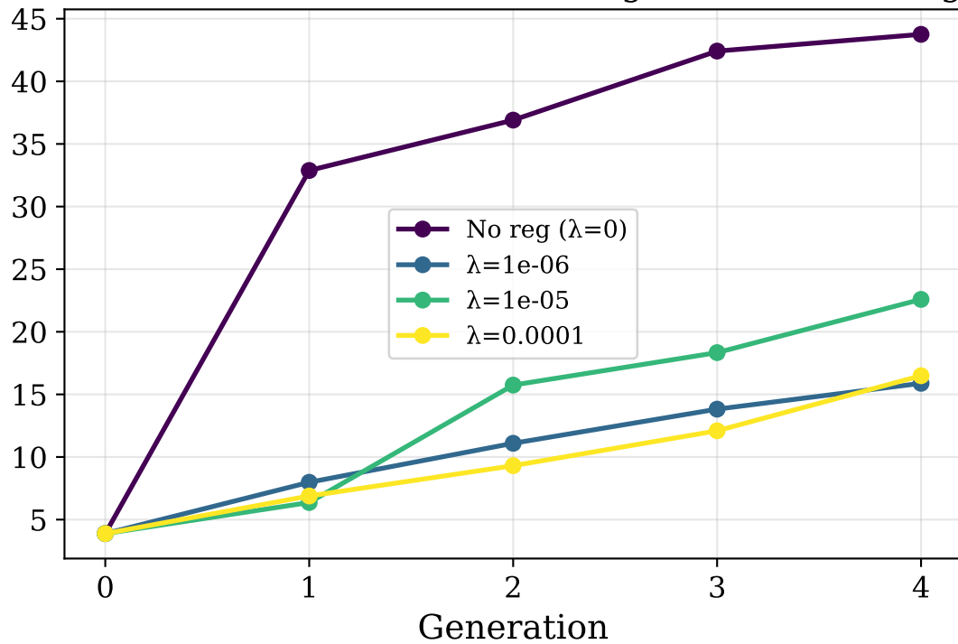
FID vs Generation for Different Regularization Strengths
