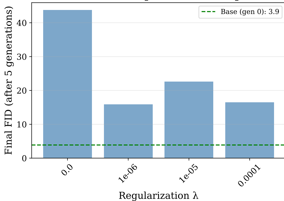
Final FID vs Regularization Strength
