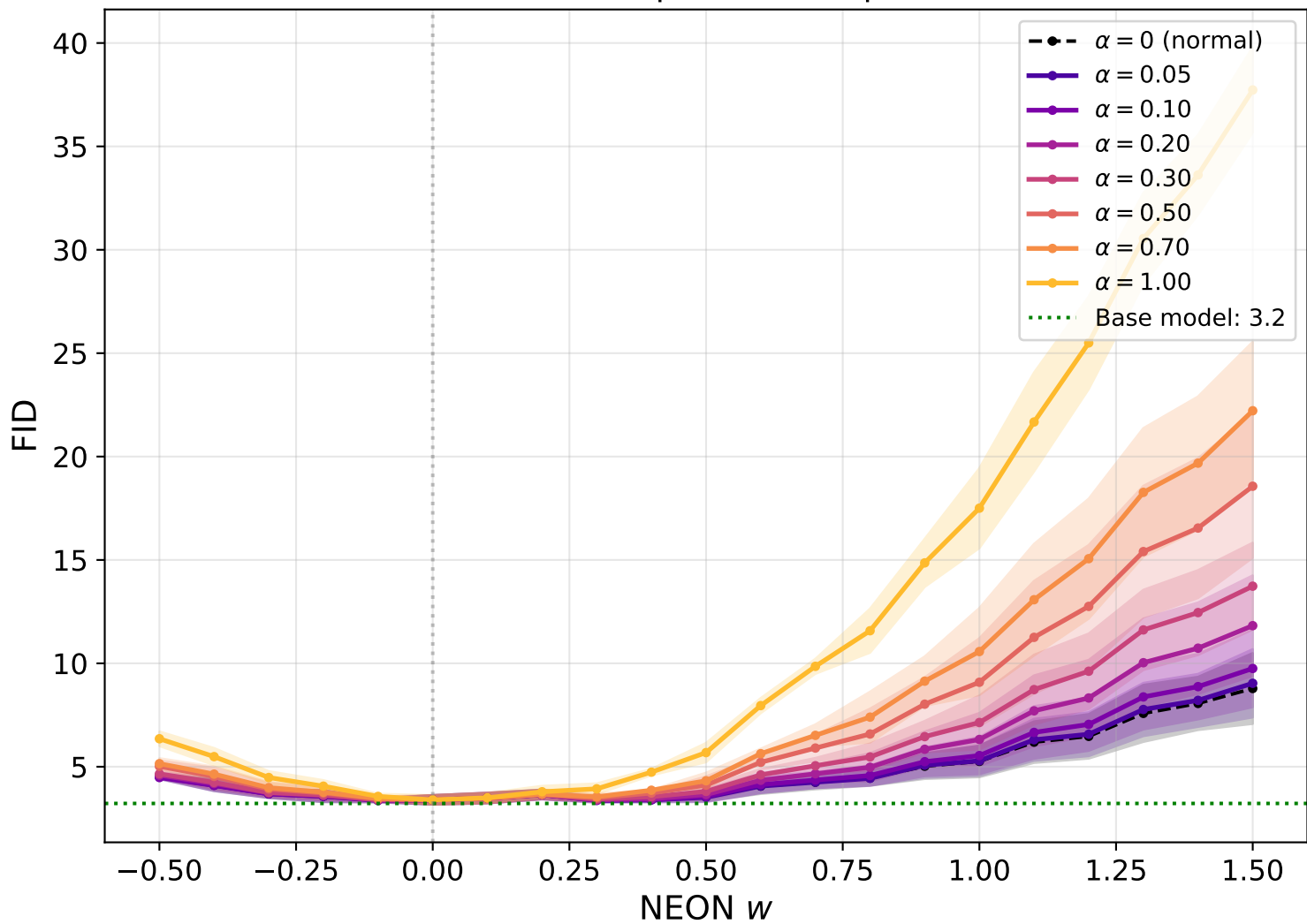
NEON with Controlled Spectral Collapse (MNIST GAN)
