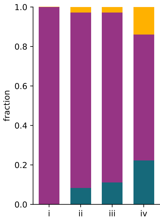
(c) 500 K
