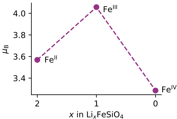
(a) Fe magnetic moments
