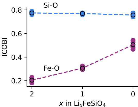
(b) (Fe/Si)-O ICOBI
