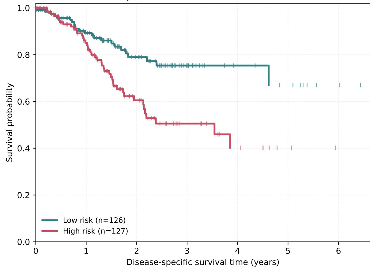
STAD | 5-seed mean-risk ensemble OOF
