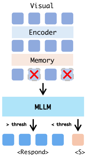
(B) <Silence>-based
