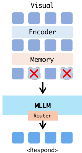
(C) Router-based
