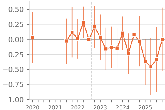
LM-AIOE exposure
