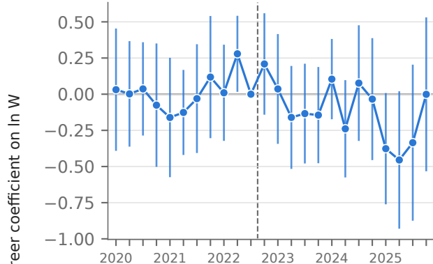
GPT-4-rated exposure
