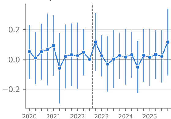
Main specification
