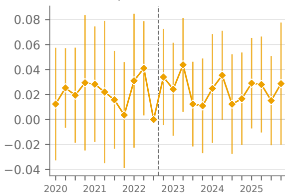
LM-AIOE exposure
