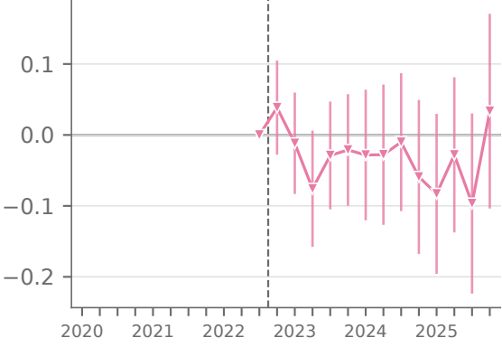
RQ1 Model 2: linear trend
