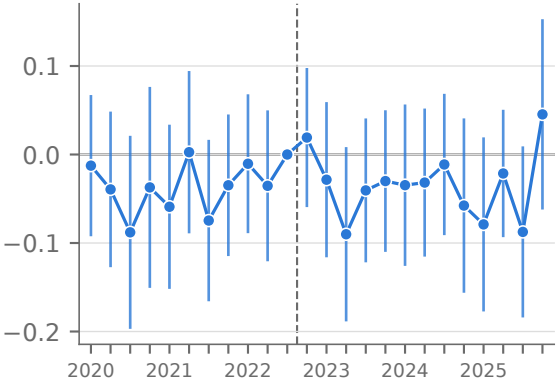
GPT-4-rated exposure
