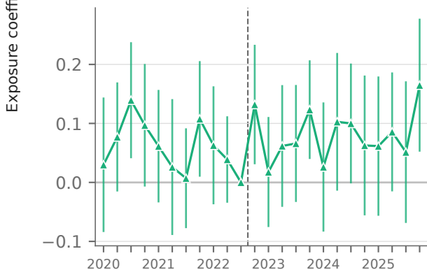
GPT-4-rated exposure
