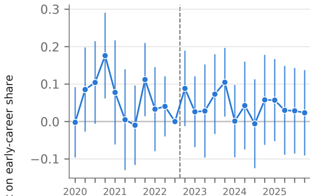
GPT-4-rated exposure
