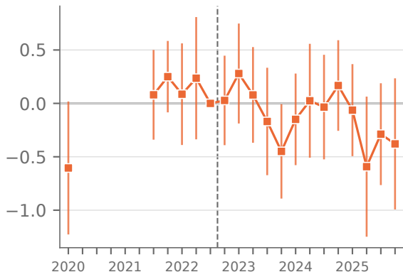
LM-AIOE exposure
