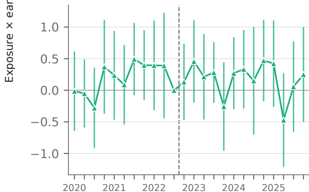
GPT-4-rated exposure
