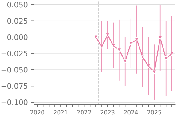
RQ1 Model 2: linear trend
