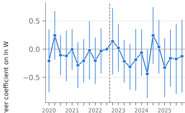
GPT-4-rated exposure
