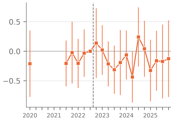
LM-AIOE exposure
