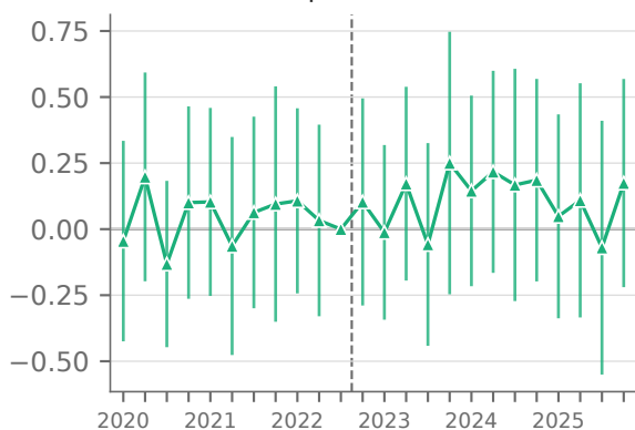
GPT-4-rated exposure
