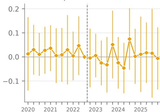
LM-AIOE exposure
