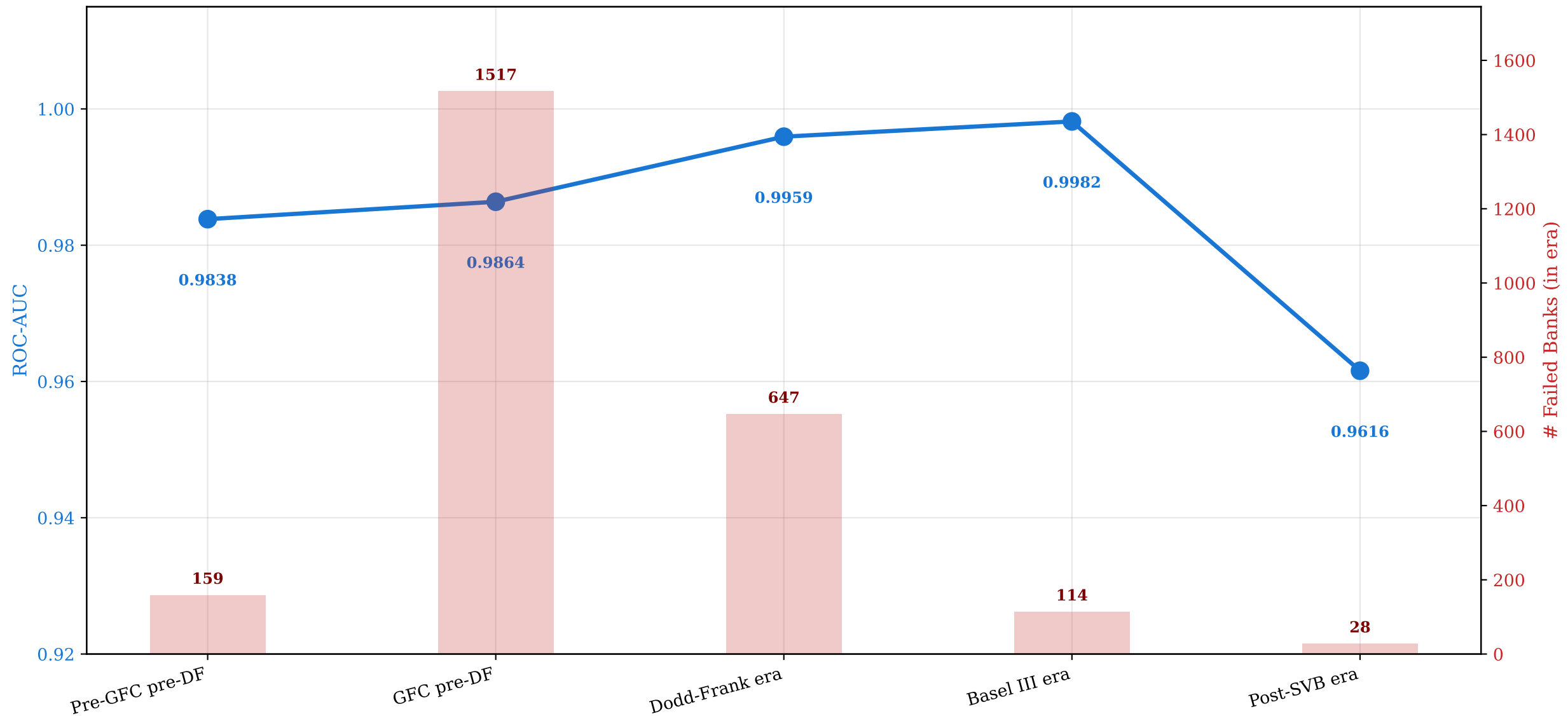
Predictive Performance by Regulatory Era (XGBoost, era-specific feature set)
