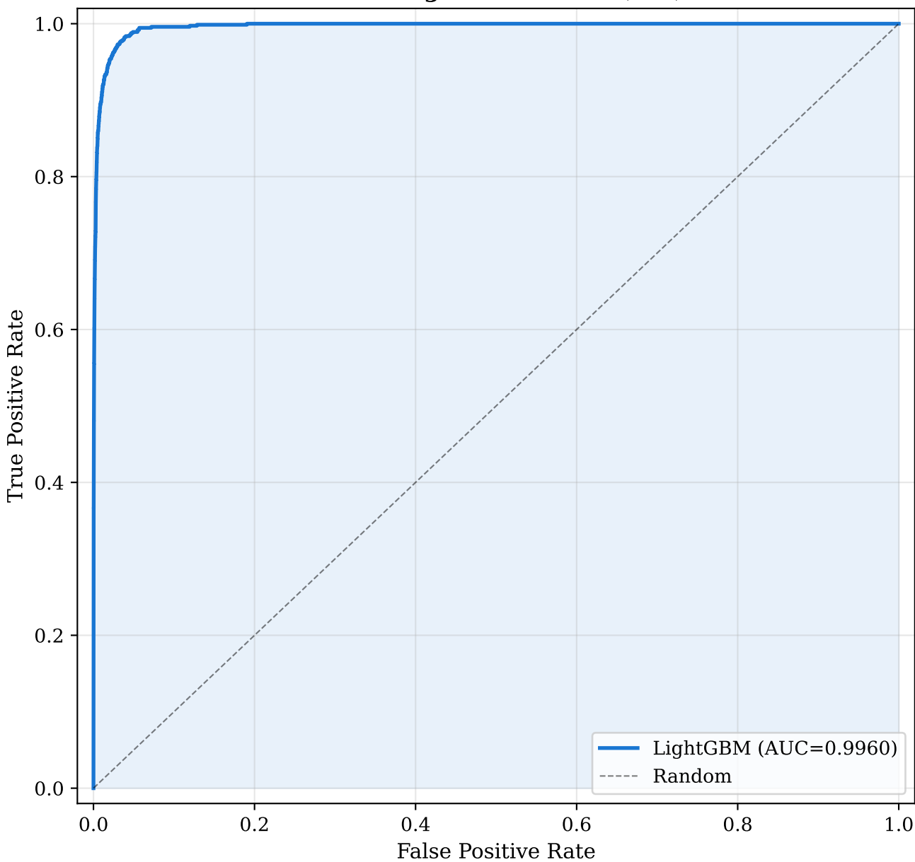
ROC Curve - LightGBM Predicting Bank Failure (t+4)
