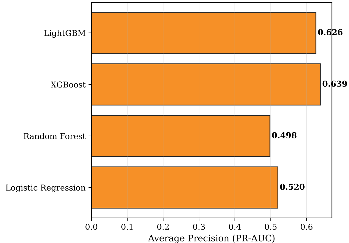
Average Precision (Class Imbalance Adjusted)
