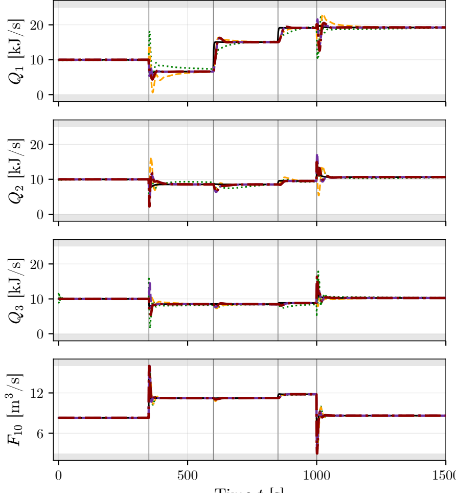
Figure 6: Closed-loop manipulated variables of the grade campaign in the original setup. The panels are Q_1 , Q_2 , Q_3 , and F_{10} . The solid black line is the nonlinear benchmark, the dotted green line is the MPC using the N4SID model, the dashed orange line is the MPC using the Koopman model with the linear decoder, the dashed purple line is the proposed formulation linearized at the current state estimate, and the dash-dotted red line is the proposed formulation linearized at the target of the previous sampling instant. The grey vertical lines mark the same grade changes and feed upsets as in Fig. 5, and the grey bands are the input bounds of Table 1.
