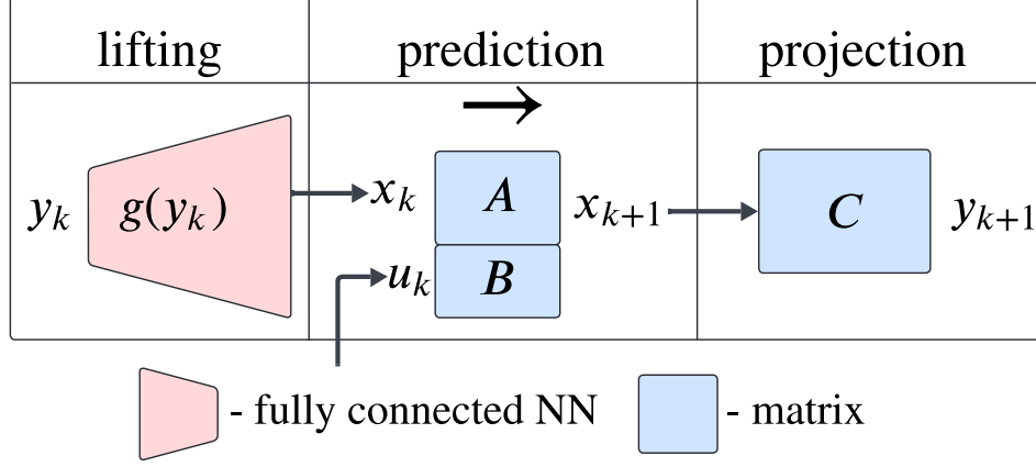
Figure 2: Architecture of the deep Koopman operator for a nonautonomous system with the linear approximation of the output map. This approximation is required for the MPC problem to remain a quadratic program.
