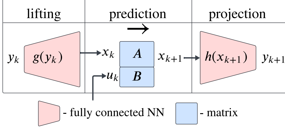
Figure 1: Architecture of the deep Koopman operator for nonautonomous systems.
