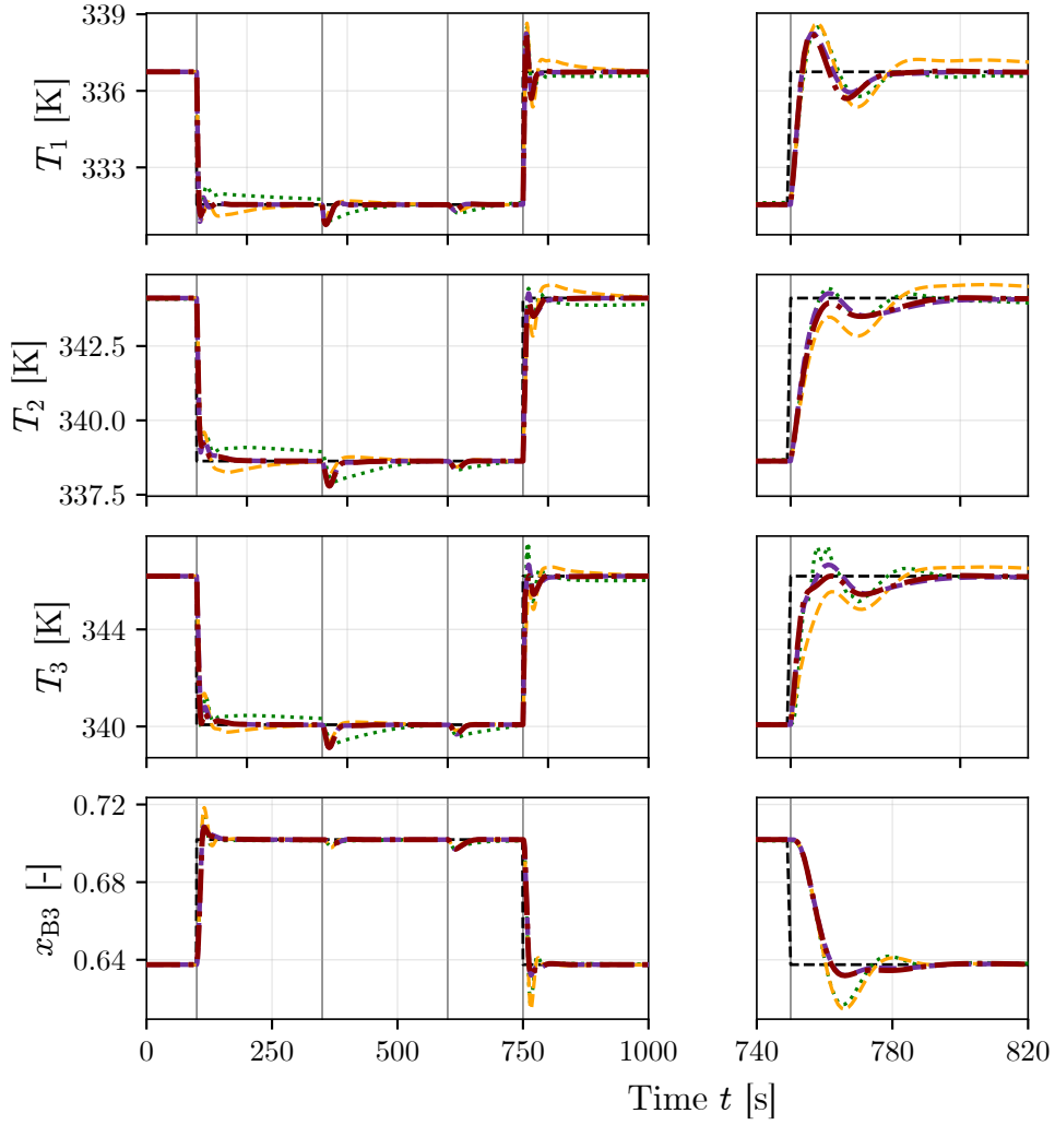
Figure 5: Closed-loop outputs of the simulation scenario. The black dashed line is the setpoint, the dotted green line is the MPC using the N4SID model, the dashed orange line is the MPC using the Koopman model with the linear decoder, the dashed purple line is the proposed formulation linearized at the current state estimate, and the dash-dotted red line is the proposed formulation linearized at the target of the previous sampling instant. The grey vertical lines mark the setpoint changes and the feed disturbances listed in Table 4.
