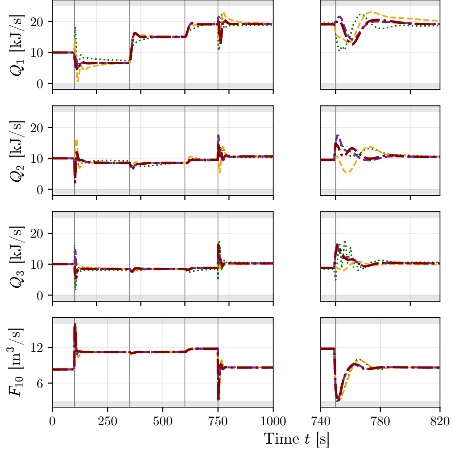
Figure 6: Closed-loop manipulated variables of the simulation scenario. The dotted green line is the MPC using the N4SID model, the dashed orange line is the MPC using the Koopman model with the linear decoder, the dashed purple line is the proposed formulation linearized at the current state estimate, and the dash-dotted red line is the proposed formulation linearized at the target of the previous sampling instant. The grey vertical lines mark the setpoint changes and the feed disturbances listed in Table 4, and the grey bands are the input bounds of Table 1.
