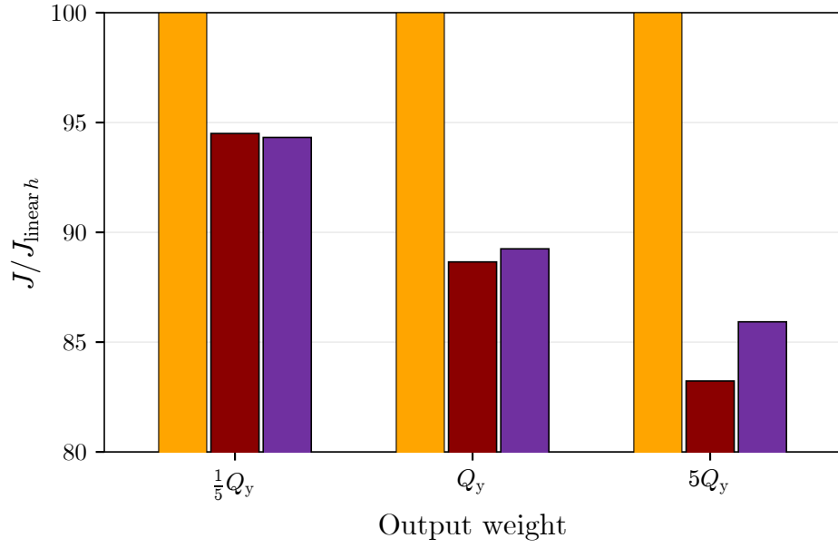
Figure 7: Closed-loop objective J divided by the objective of the Koopman controller with the linear decoder at the same tuning. The orange bars are the linear decoder, the red bars the proposed formulation linearized at the previous target, and the purple bars the proposed formulation linearized at the current state estimate.
