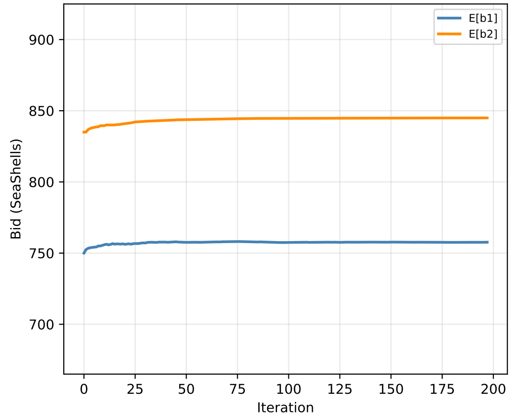
Fictitious Play
