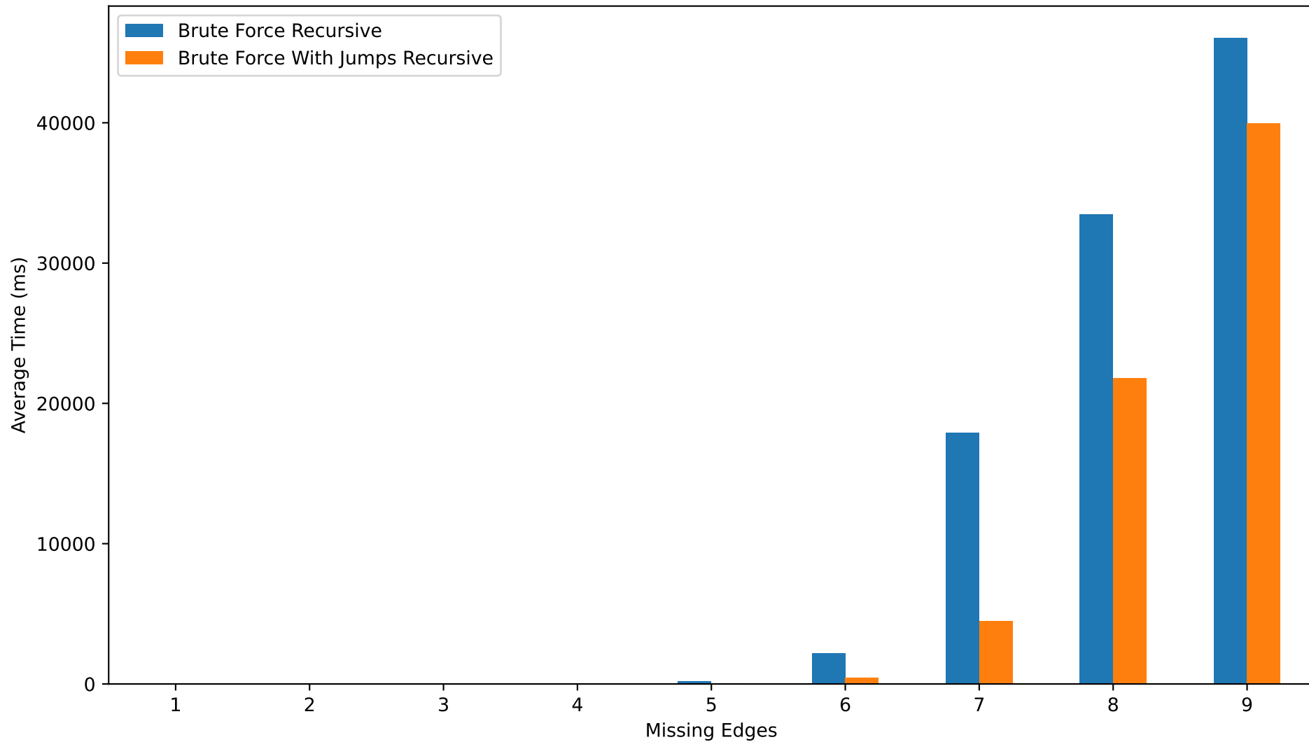
Average Time vs. Missing Edges
