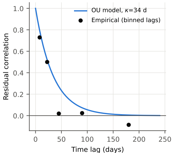
(a) Temporal correlation of residuals
