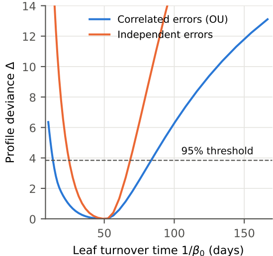
(b) Profile likelihood of the leaf turnover time
