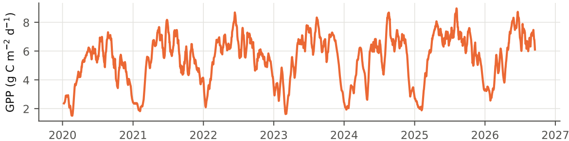
(c) Ground-area GPP (15-d mean)
