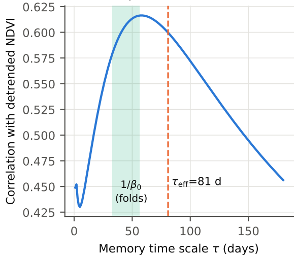
(a) Memory scan
