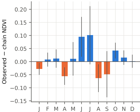
(b) Seasonal structure of the discrepancy
