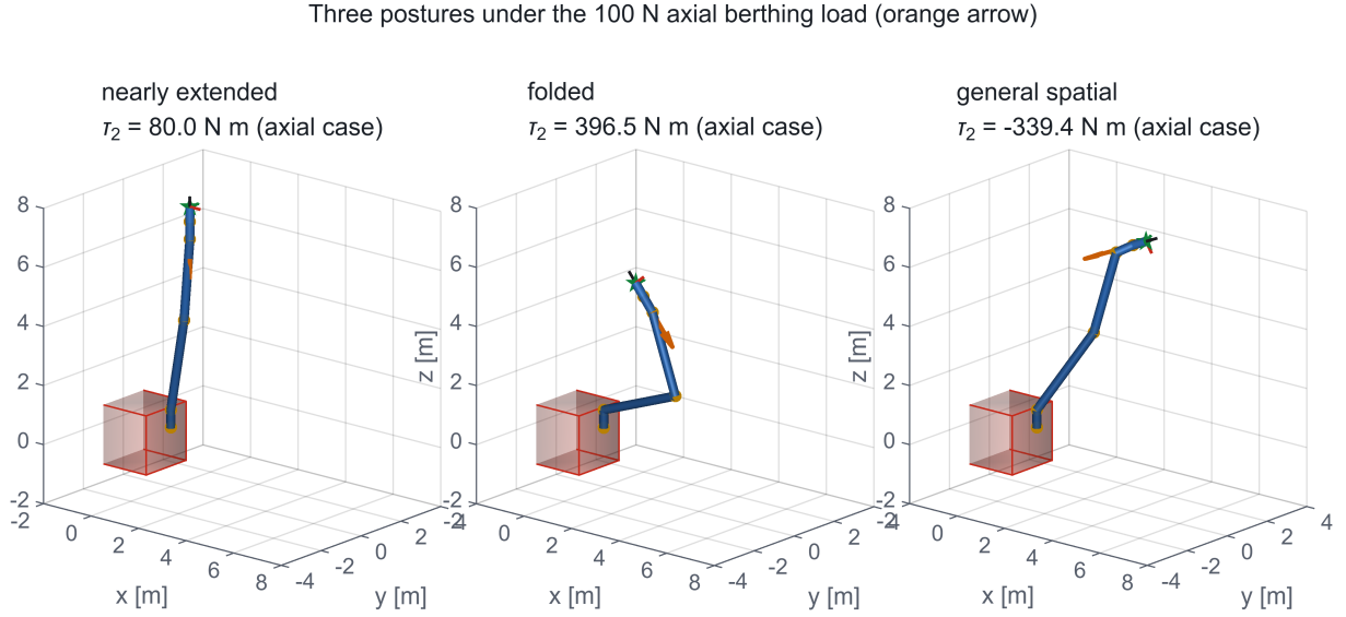
Figure 8: The three study postures under the 100 N axial berthing load (arrow). Shoulder torque rises fivefold from the extended to the folded configuration for an identical applied force.
