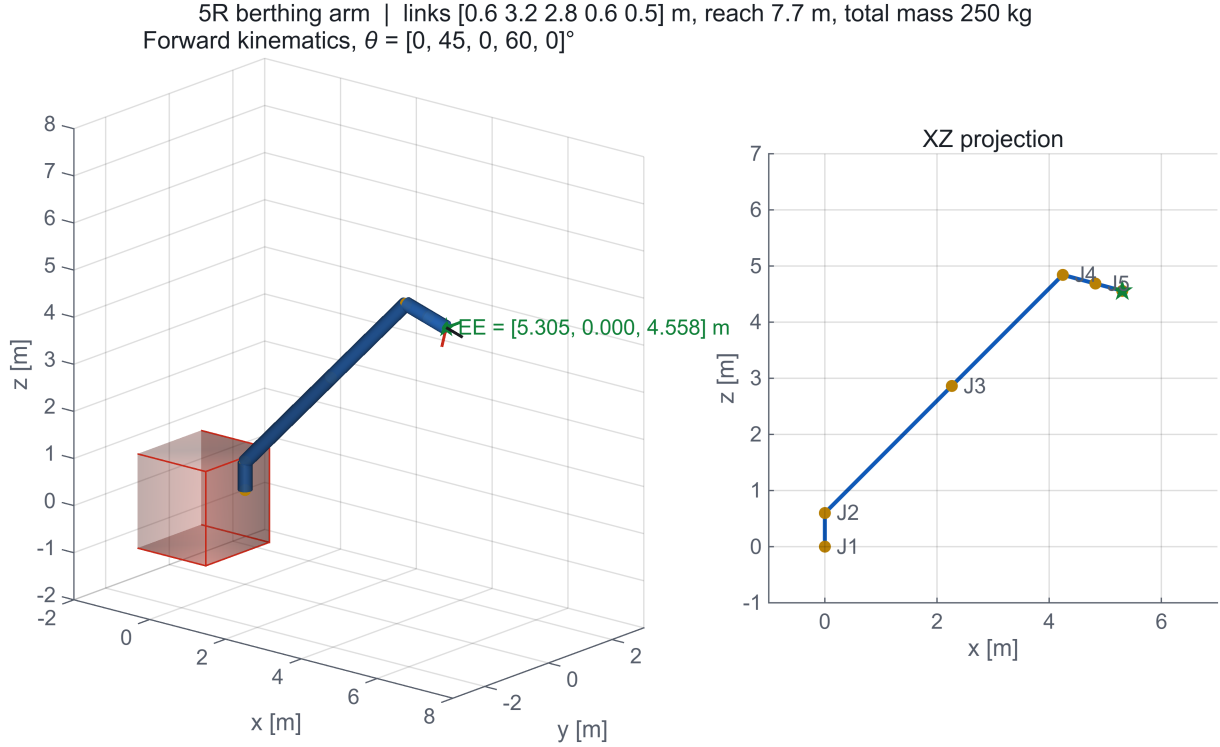
Figure 7: Forward kinematics at the acceptance pose. Left: three-dimensional rendering with the end-effector triad. Right: xz projection with the joint origins labelled. Reach at this pose is 6.99 m of the 7.7 m maximum.
