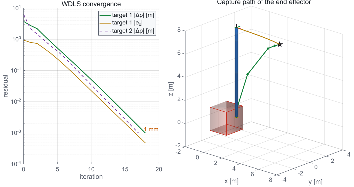
Figure 9: Left: WDLs convergence for both targets, log scale. Position residual falls below 1 mm in 18 iterations. Right: the capture path of the end effector from the stowed pose to the solution, with the final configuration overlaid.
