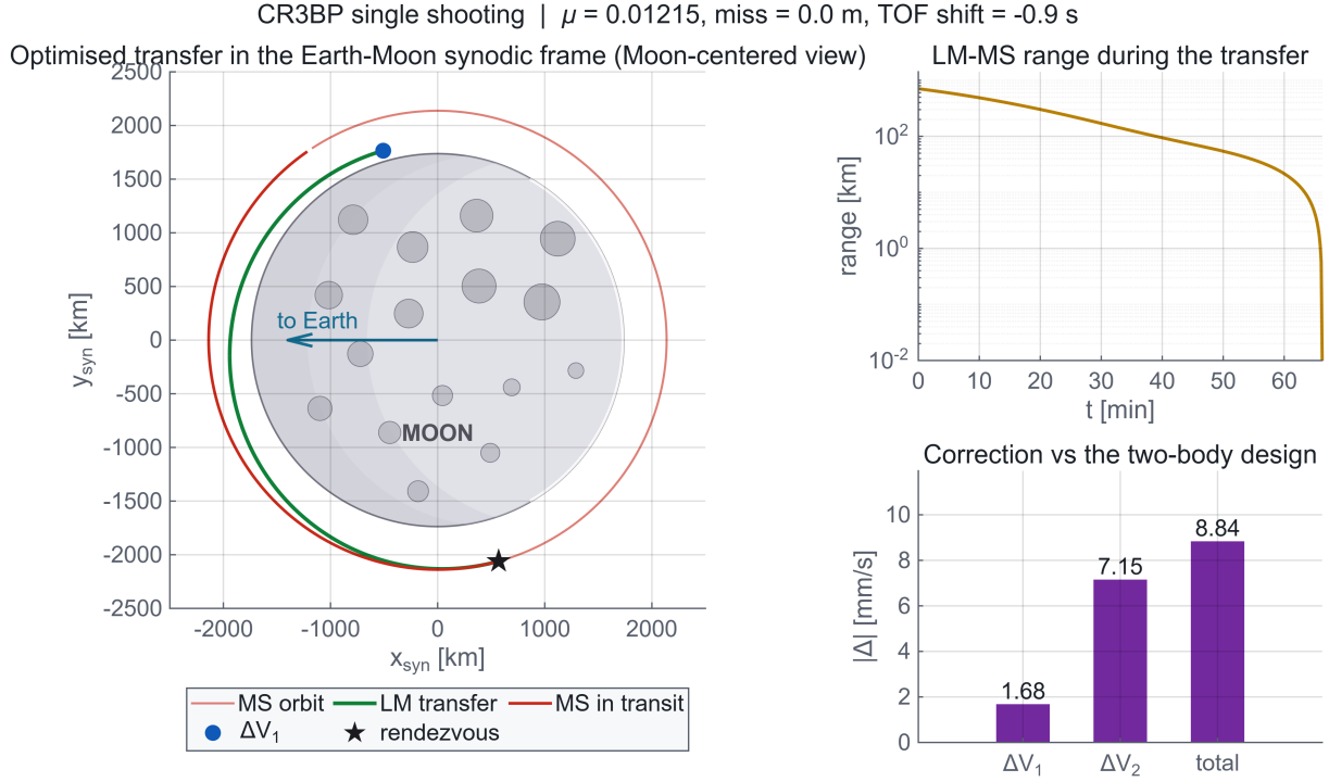
Figure 6: Optimised transfer in the Earth-Moon synodic frame, Moon-centred view. The arc is the same climb as Figure 1 seen from a rotating frame. Right: range history and the correction relative to the two-body design, in millimetres per second.
