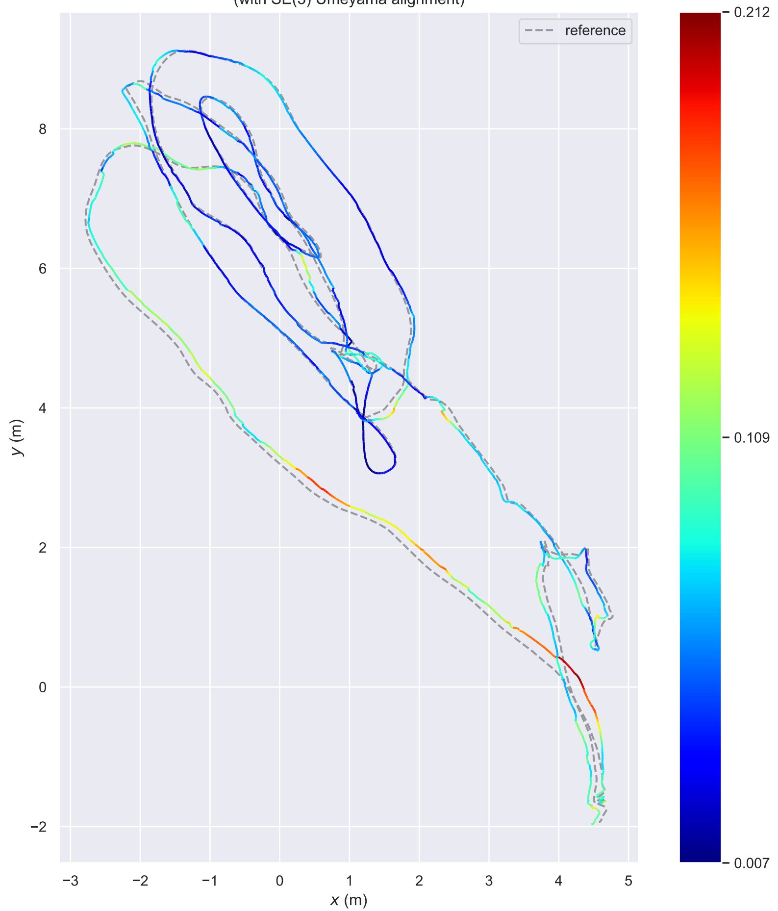
APE w.r.t. translation part (m) (with SE(3) Umeyama alignment)
