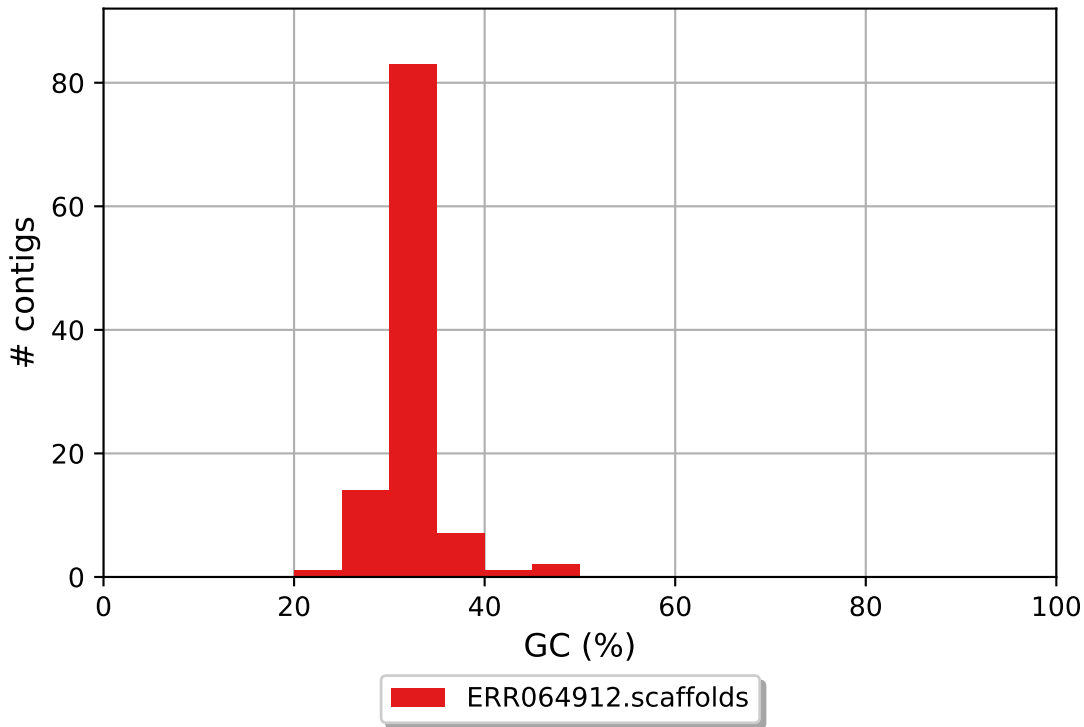
ERR064912.scaffolds GC content
