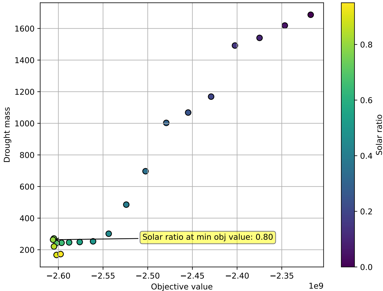
Objective value vs drought mass, with respect to solar ratio (0.3 Dunkleflaute)
