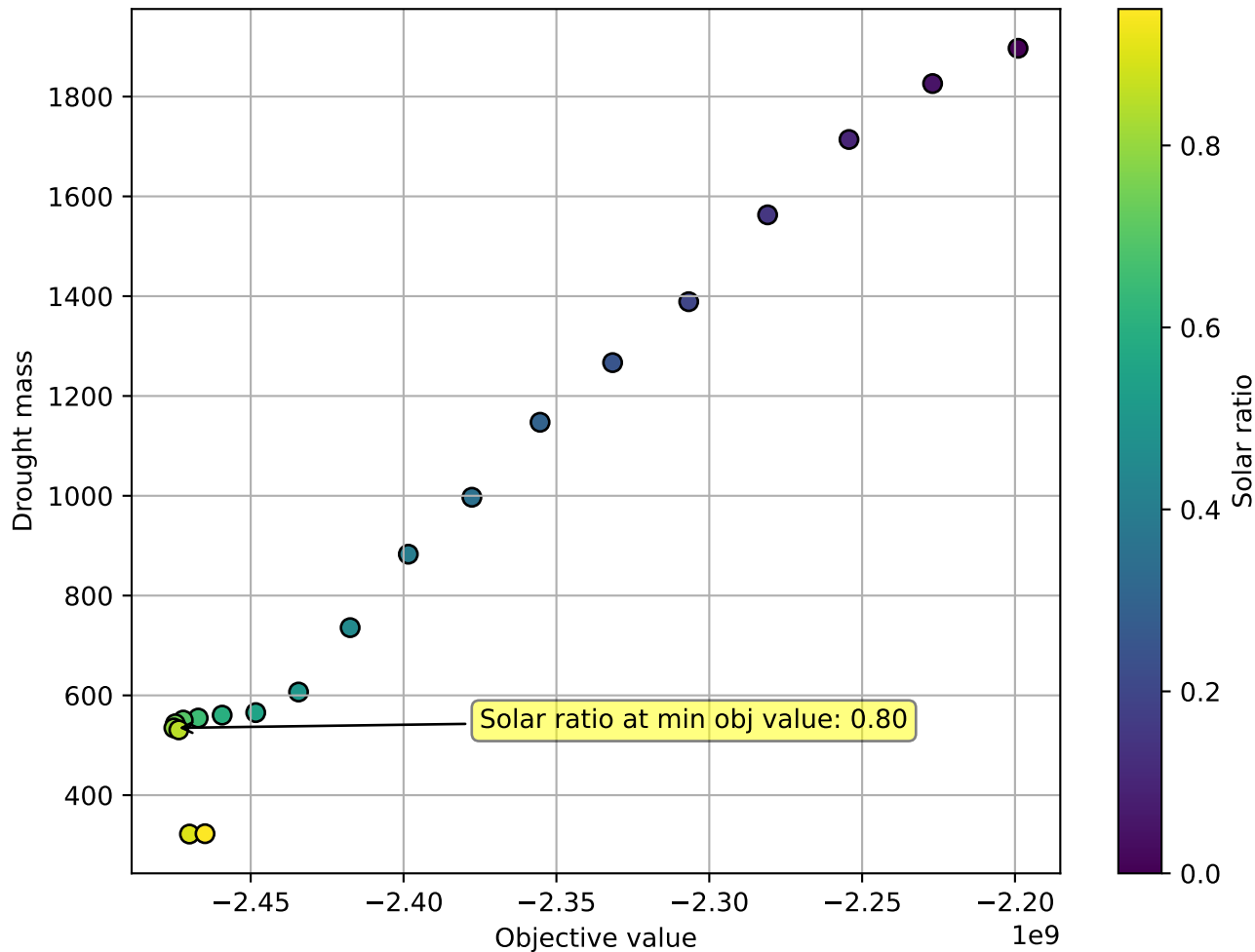
Objective value vs drought mass, with respect to solar ratio (0.8 Dunkleflaute)
